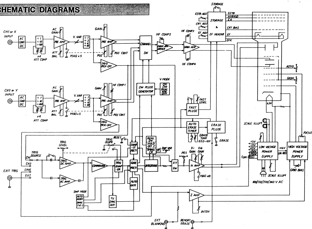
BLOCK DIAGRAM 1
