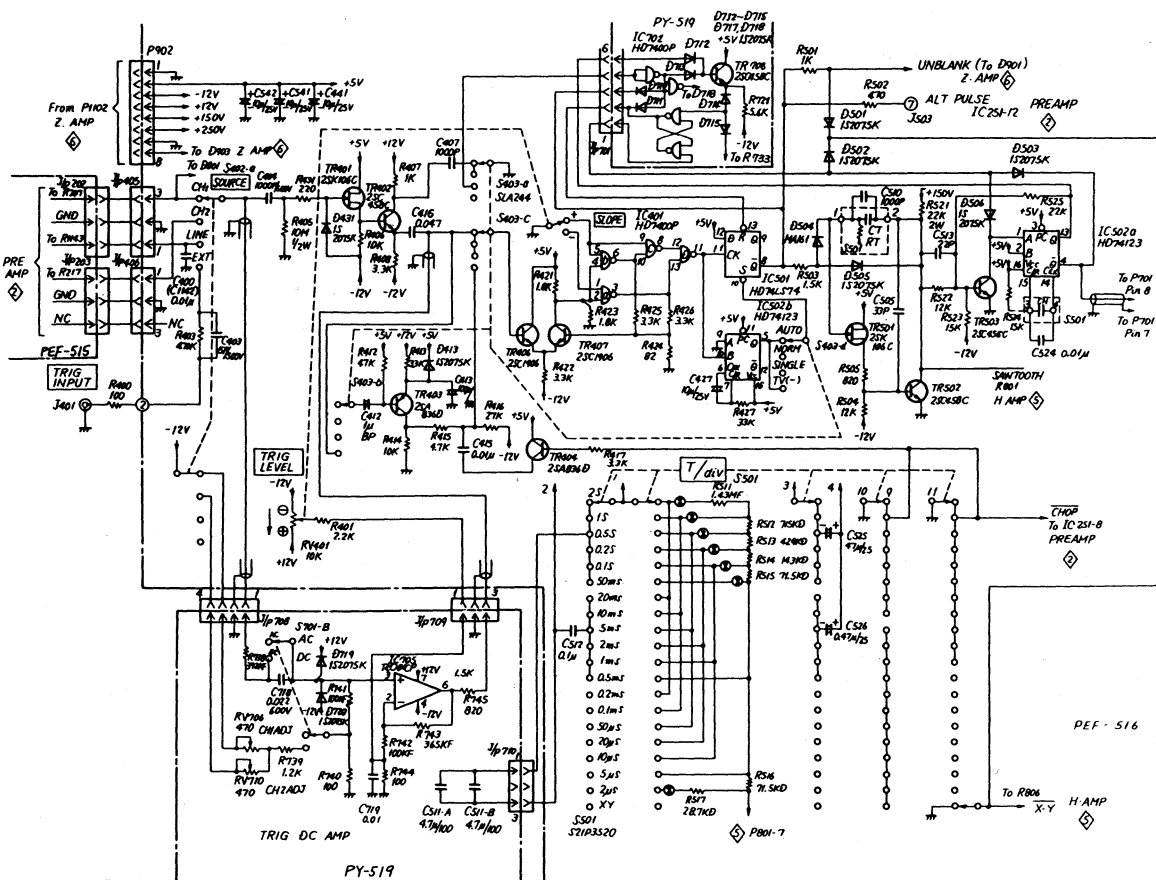
TRIGGER & SWEEP 4
