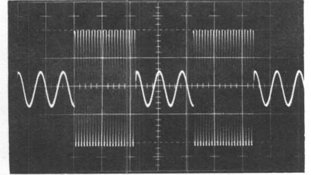
AM/FSK MODULATION
