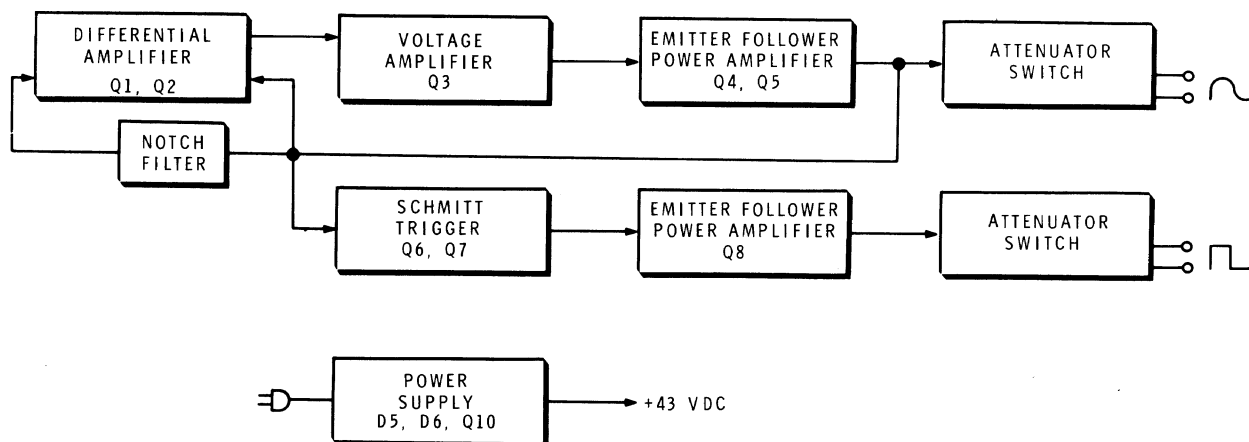
BLOCK DIAGRAM
