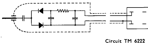
Circuit TM 6222
