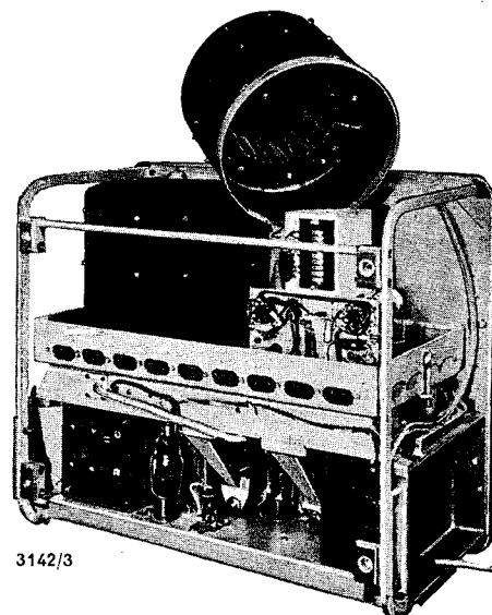
3142/3 Rear view of instrument with r.f. cover and one turret removed
