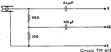
Circuit TM 6123
