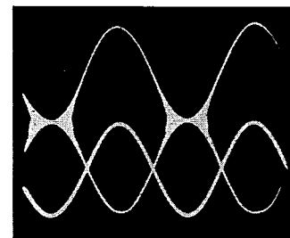
3142/13 320-kc/s carrier modulated at 400 c/s; input on lower beam
