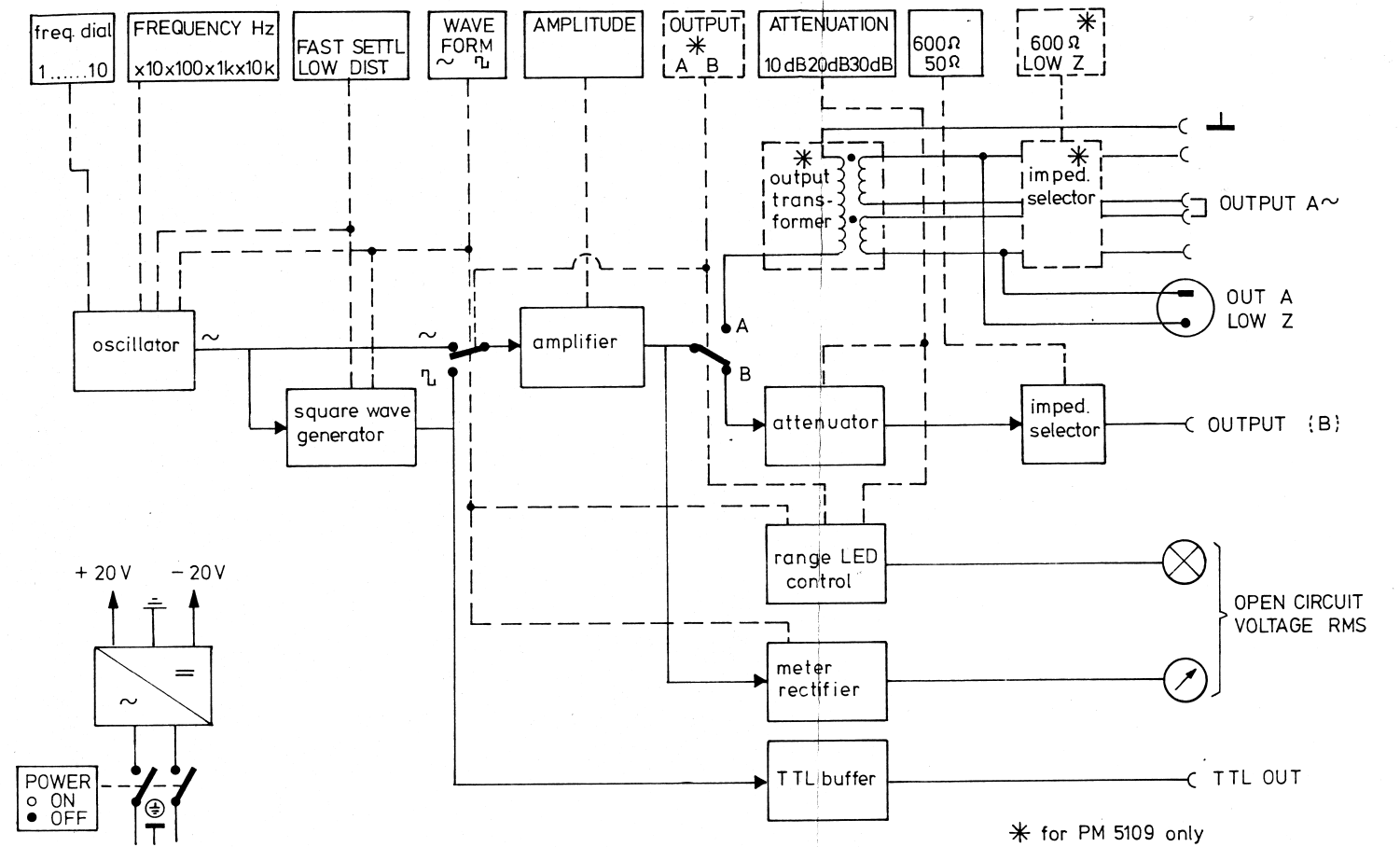
Fig. 30 Block diagram PM 5109/PM 5109 S
