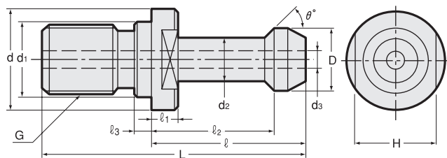
Center- thru compliant
