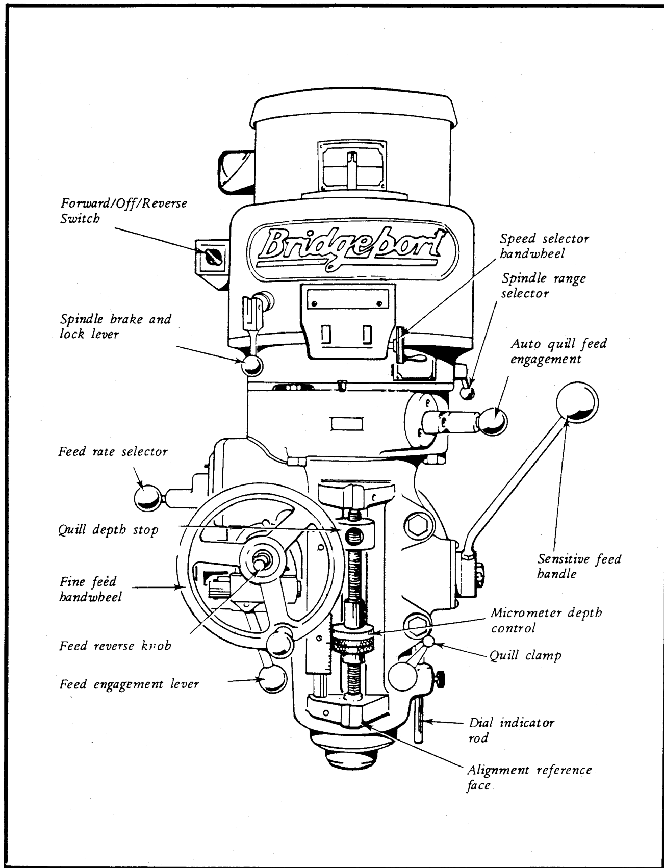
2.3 2J2 - Head Controls
