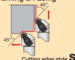
Cutting edge style S
