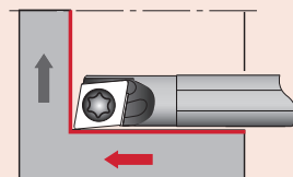
Cutting edge style X
