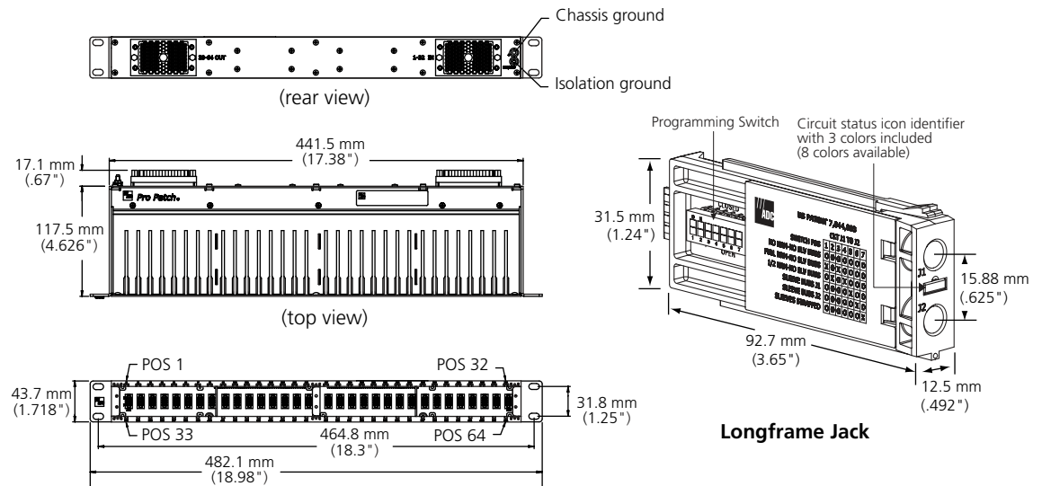
Typical 1 RU 32-Position Panel
