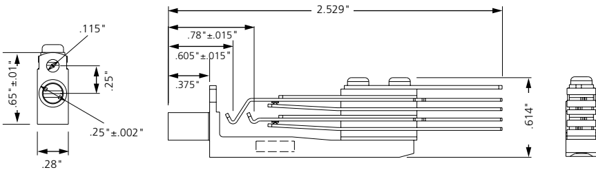
Three-Conductor Single Bantam Jack
