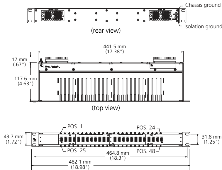
Typical 1 RU 24-Position Panel
