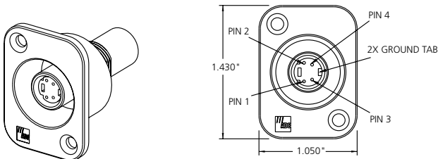
Recessed S-Video Connector (SV-R-X)
