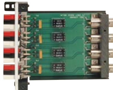
Precision Transformers, Glass Epoxy Circuit Board, True 75 \Omega BNC Connectors
