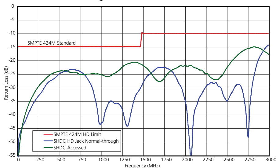
Gated Return Loss High-Performance SHDC LCC Jack
