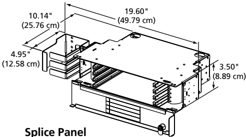
Splice Panel (48-fiber Capacity module shown)
