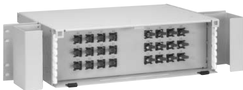
24-Position Termination/Splice Panel (front view)
