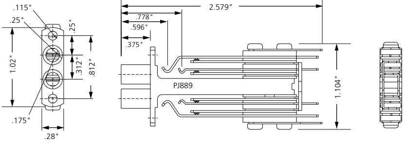
Three-Conductor Dual Bantam Jack
