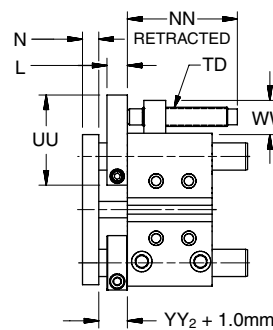
Shock Absorber Retract
