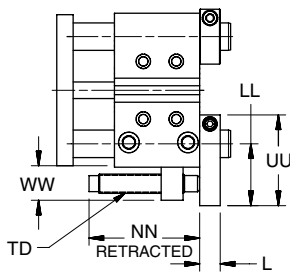
Shock Absorber Extend
