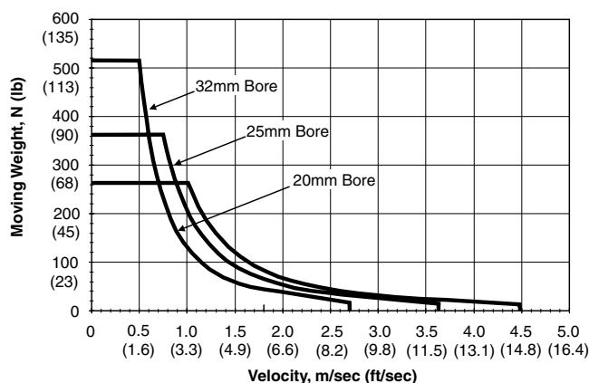
Kinetic Energy Capacity of Unit with Shock Absorbers
