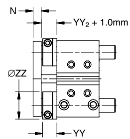
Bumpers & Adj. Stop Collars Retract
