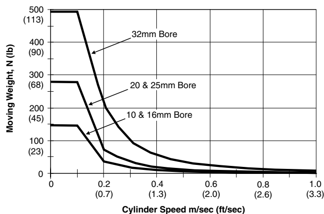
Bumper Absorption Capacity
