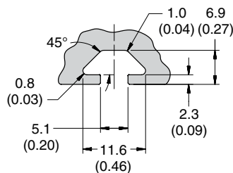
T-Slot Detail
