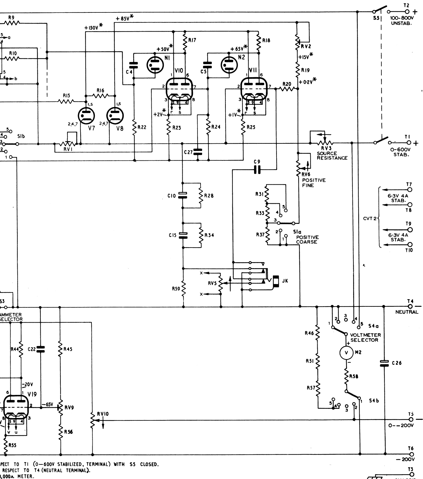
CIRCUIT DIAGRAM
