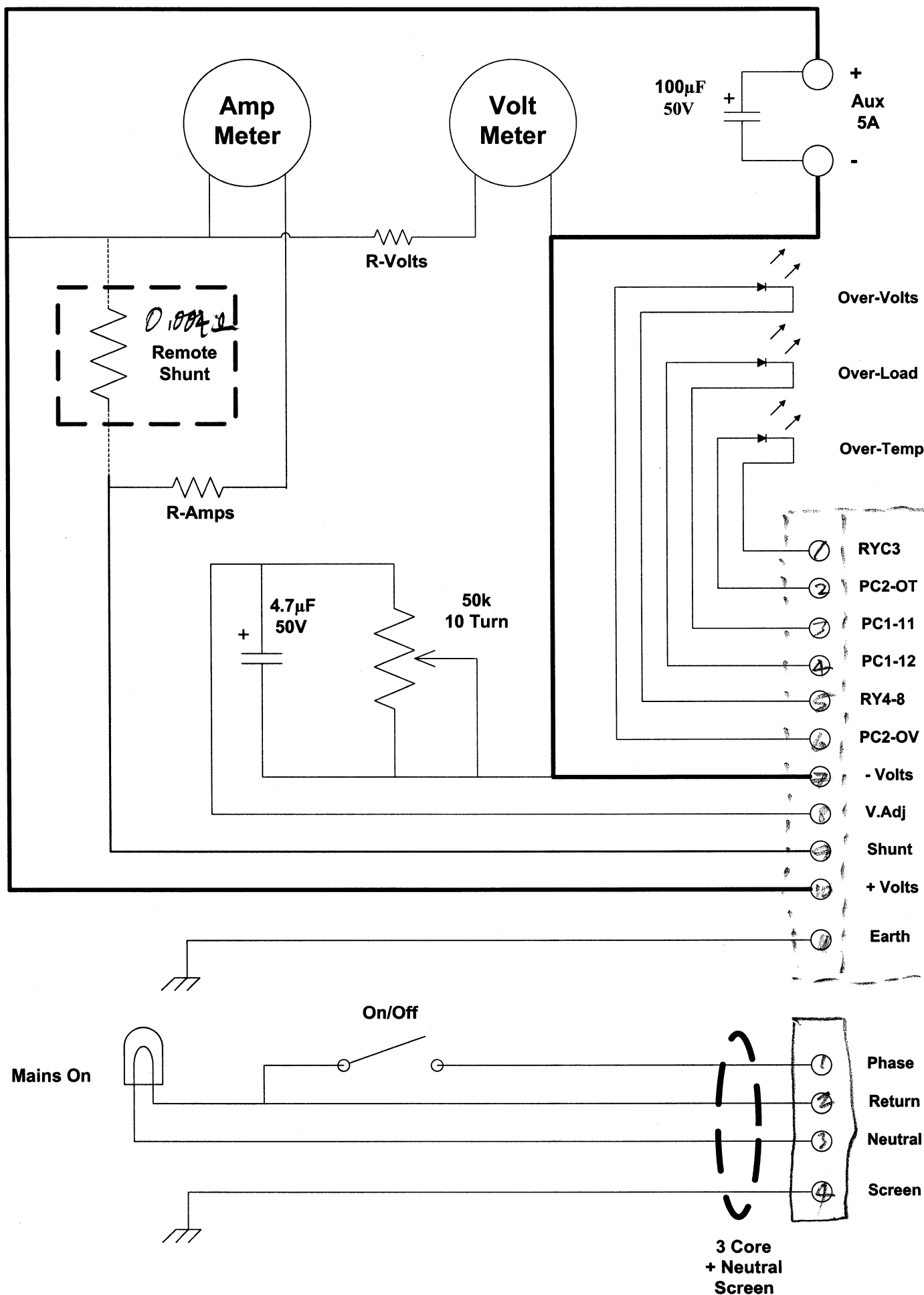
Remote Control Schematic for Redfern ASR40
