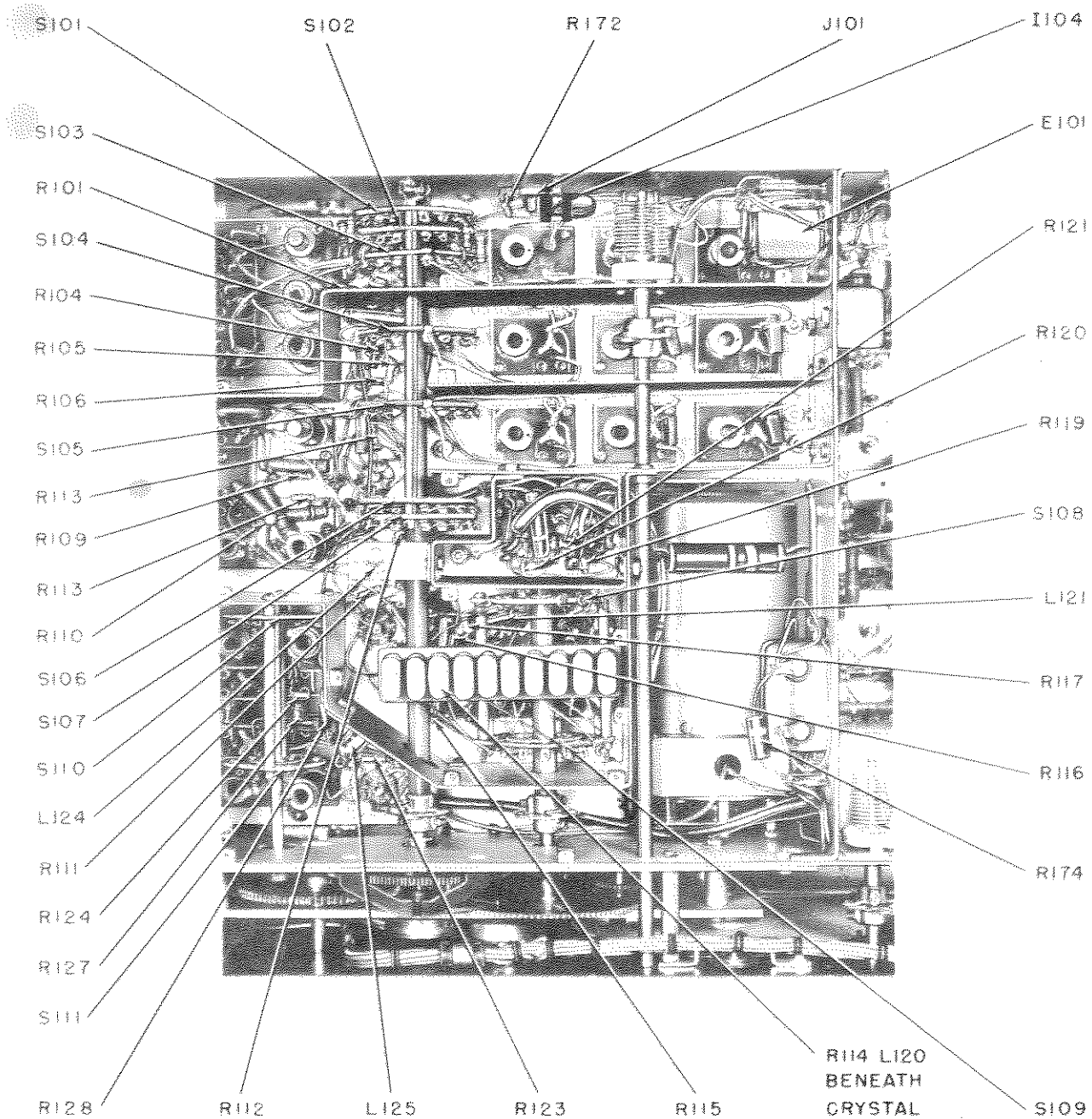
Figure 7-4. 51J-3 Bottom View, Compartment 1, Other Components
