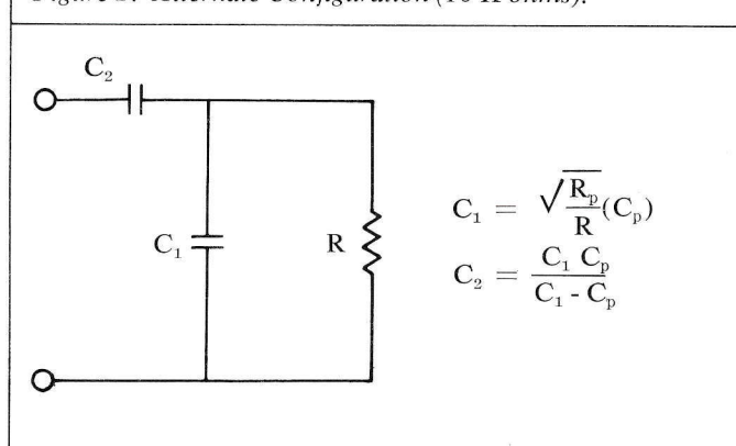
Figure 2. Alternate Configuration (10 K ohms).
