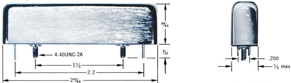
Case Style V
