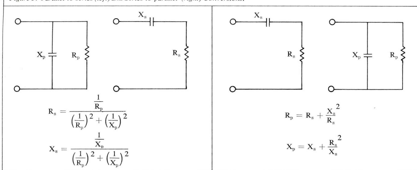
Figure 3. Parallel-to-series (left) and Series-to-parallel (right) Conversions.
