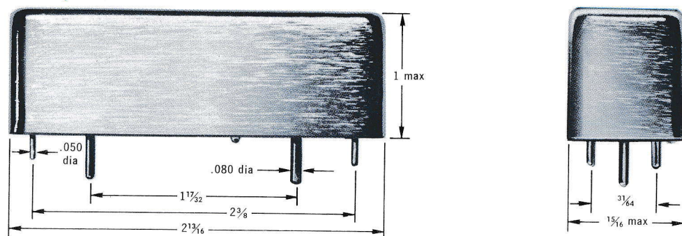
Case Style F
