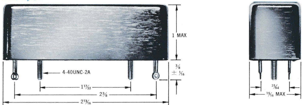
Case Style FA
