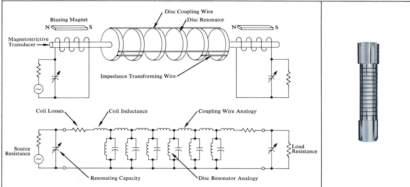
Figure 3. Mechanical Filter Electrical Analogy.
