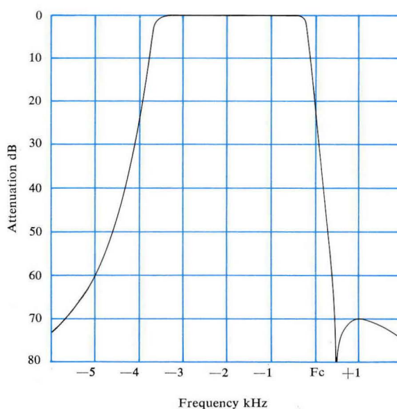
Figure 2. Frequency Response Characteristics of a Typical Voice Channel Filter.
