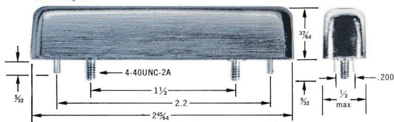
Case Style V
