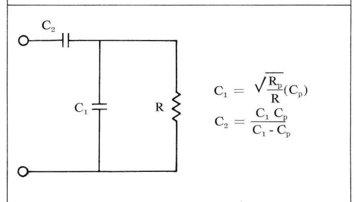
Figure 2. Alternate Configuration (10 K ohms).
