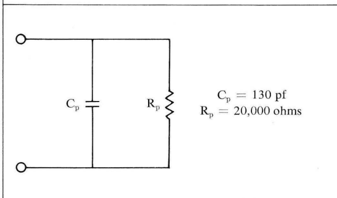
Figure 1. Specified Termination (20 K ohms).
