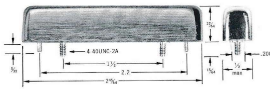
The new filters are packaged in an hermetically-sealed, plated brass case. Provides own studs for mounting.
