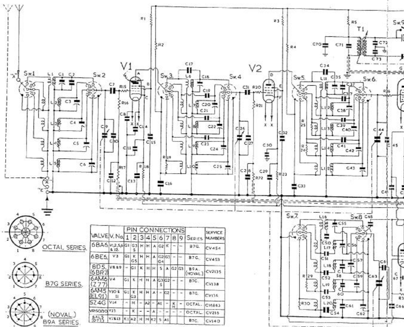
FIGURE 1. Circuit diagram
