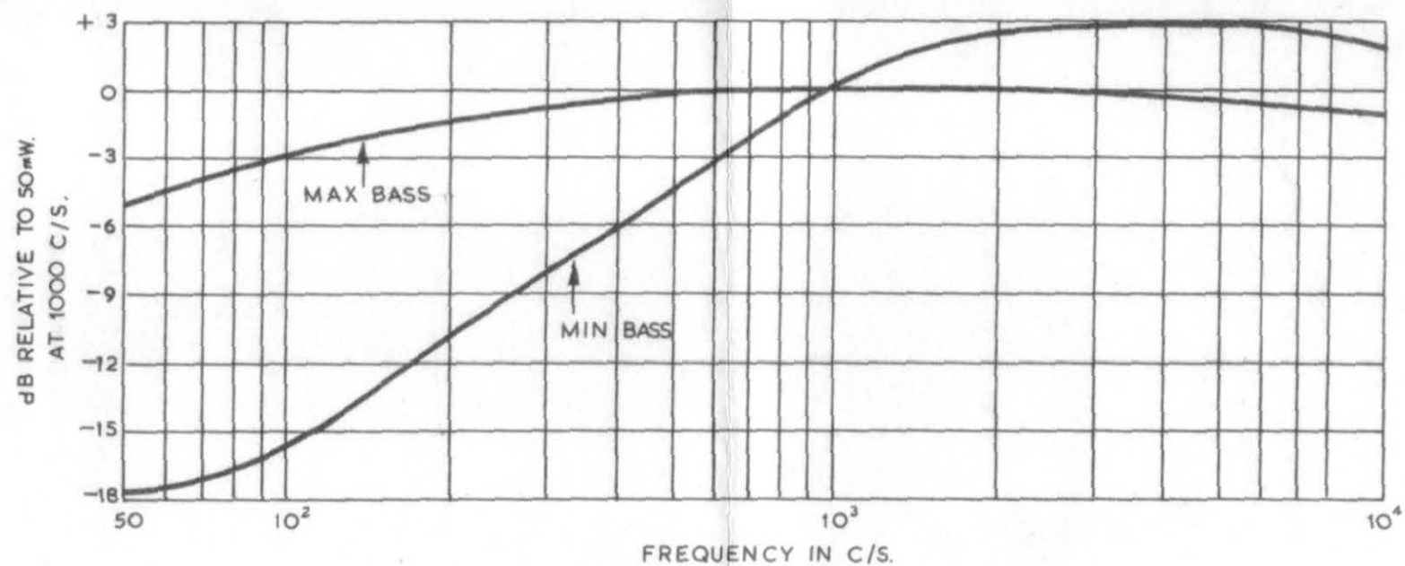
AUDIO RESPONSE IN MAXIMUM AND MINIMUM POSITIONS OF BASS SWITCH. (AUDIO FILTER OUT OF CIRCUIT AND VOLUME CONTROL AT MAX.)
