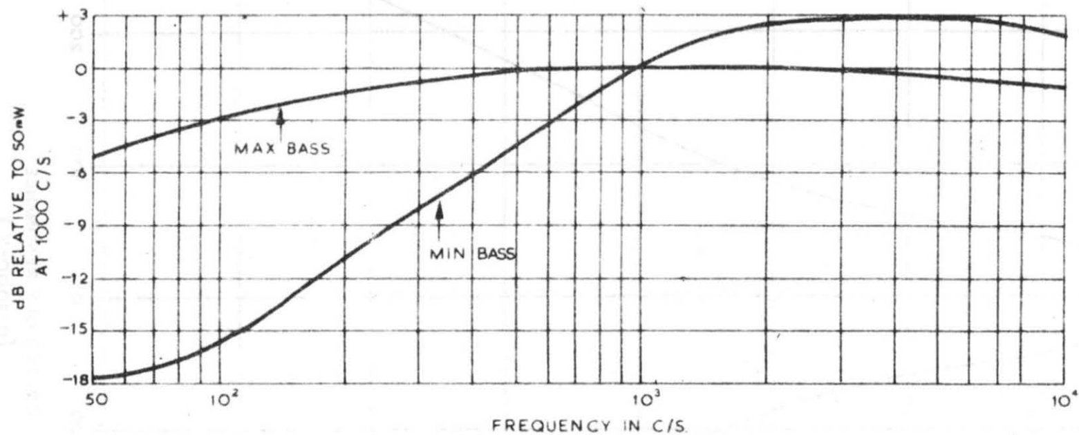
FIG 1. AUDIO RESPONSE IN MAXIMUM AND MINIMUM POSITIONS OF BASS SWITCH. (AUDIO FILTER OUT OF CIRCUIT AND VOLUME CONTROL AT MAX)
