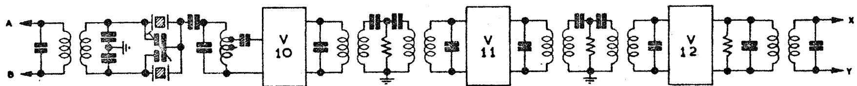
S2 AT POSITION 1 "CRYSTAL WITH AUDIO FILTER" AND POSITION 2 "CRYSTAL."
