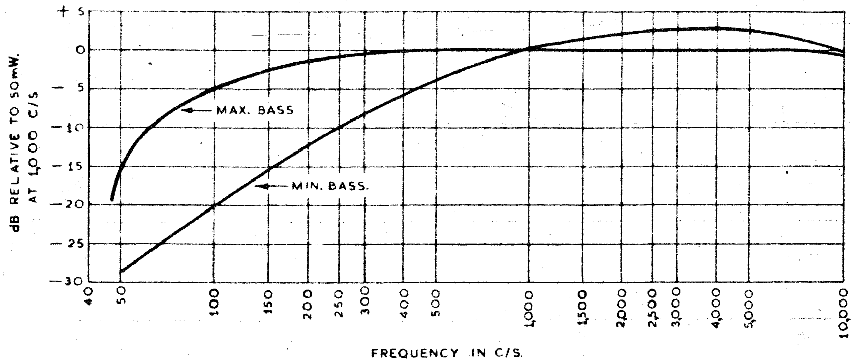
FIG.1. AUDIO RESPONSE IN MAXIMUM AND MINIMUM POSITIONS OF BASS SWITCH. (AUDIO FILTER OUT OF CIRCUIT AND VOLUME CONTROL AT MAX.)
