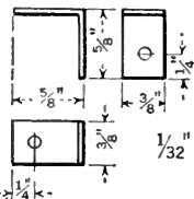
COIL MOUNTING PART No. 3
