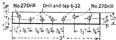
COIL MOUNTING PART No. 1
