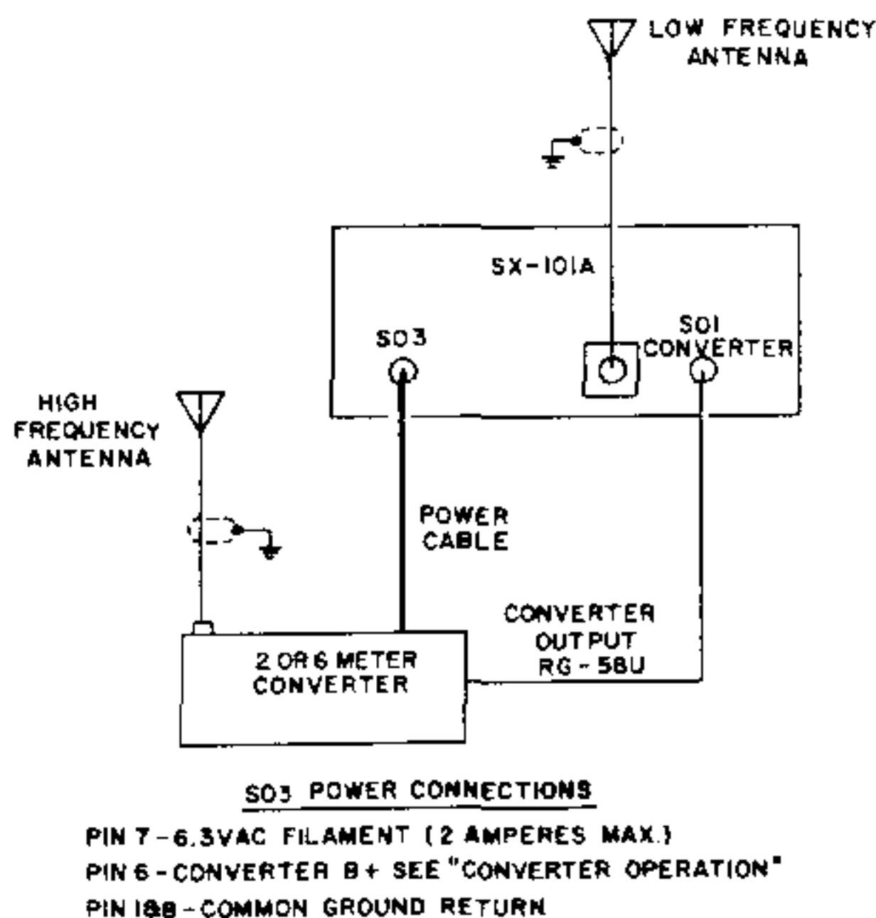
Figure 5. Converter Hookup
