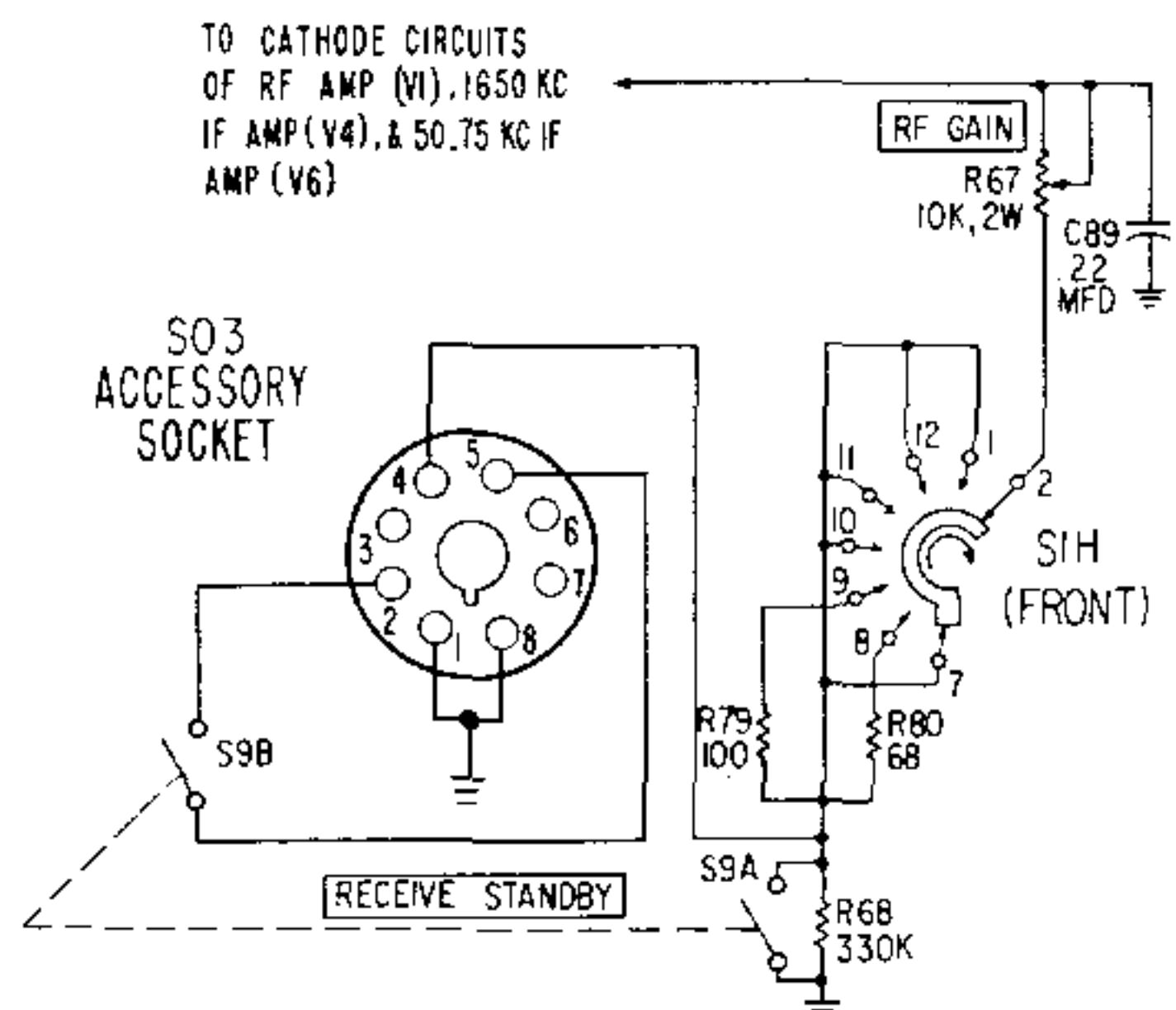
Figure 6. Simplified Sensitivity and Receive-Standby Circuits
