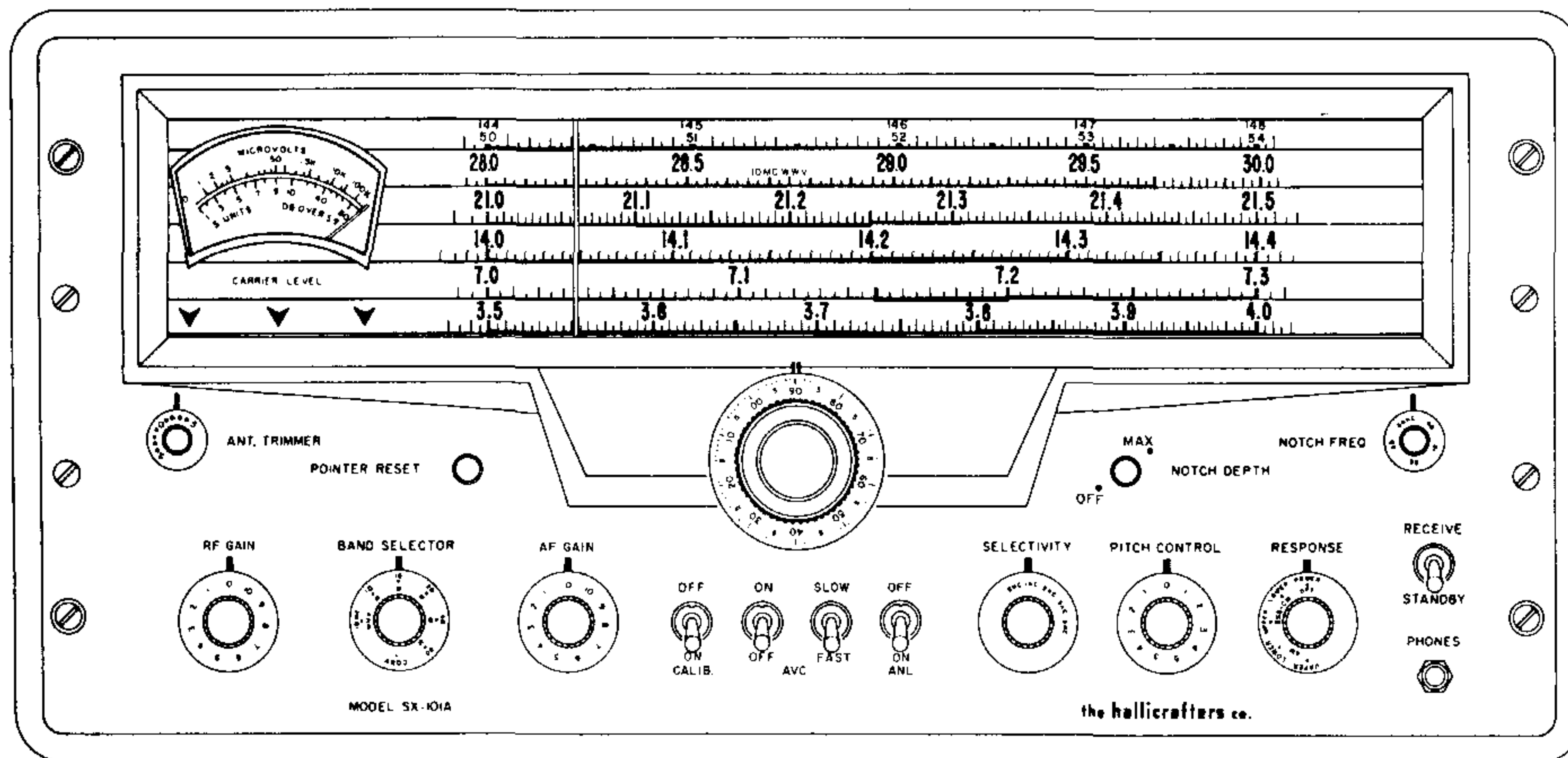
Figure 7. Operating Controls
