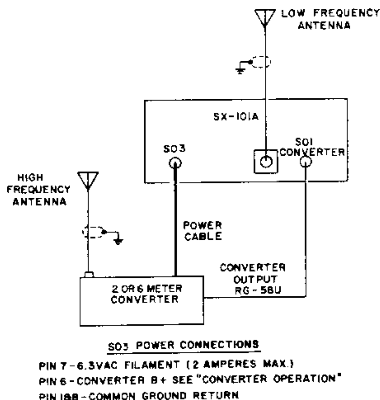
Figure 5. Converter Hookup
