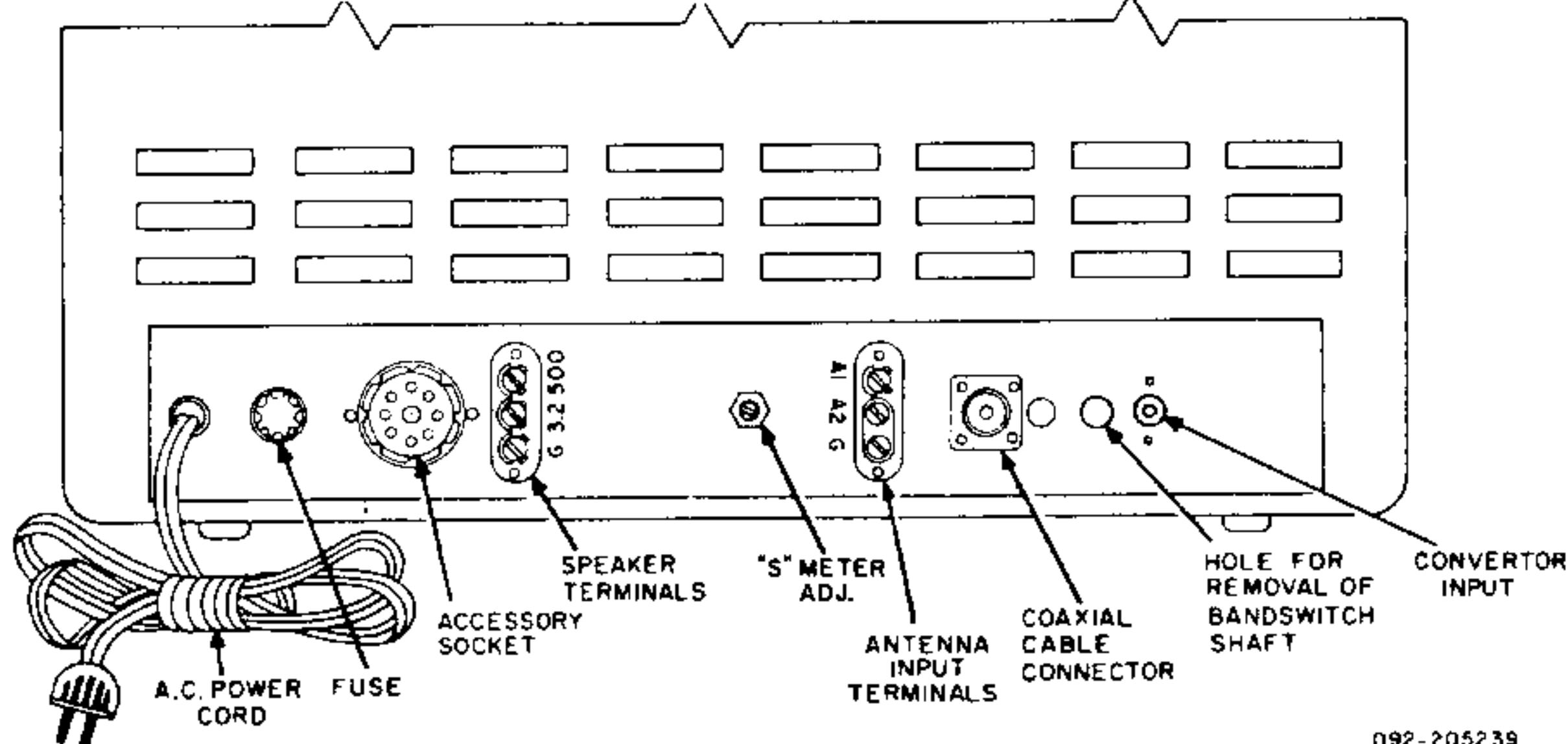
Figure 4. Rear View of Receiver
