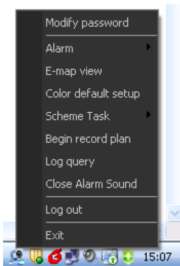
Figure 3-100 Tray Menu
