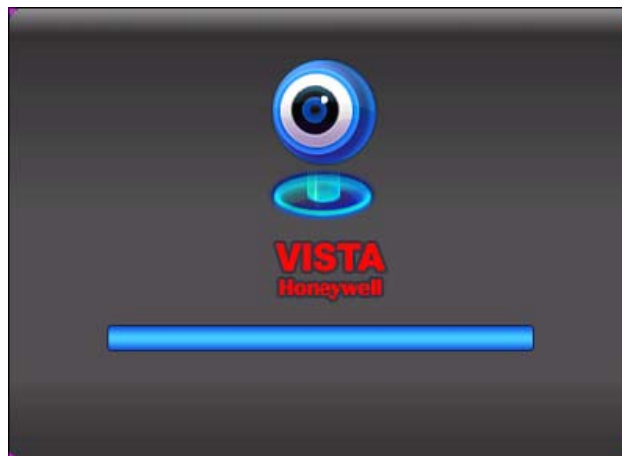
Figure 3-2 Initialization Interface
