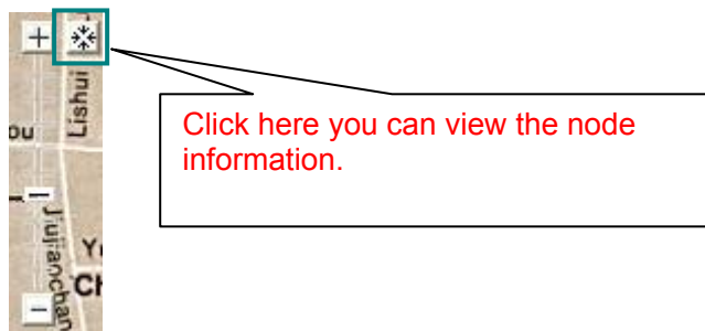
Figure 3-20 Node Information
