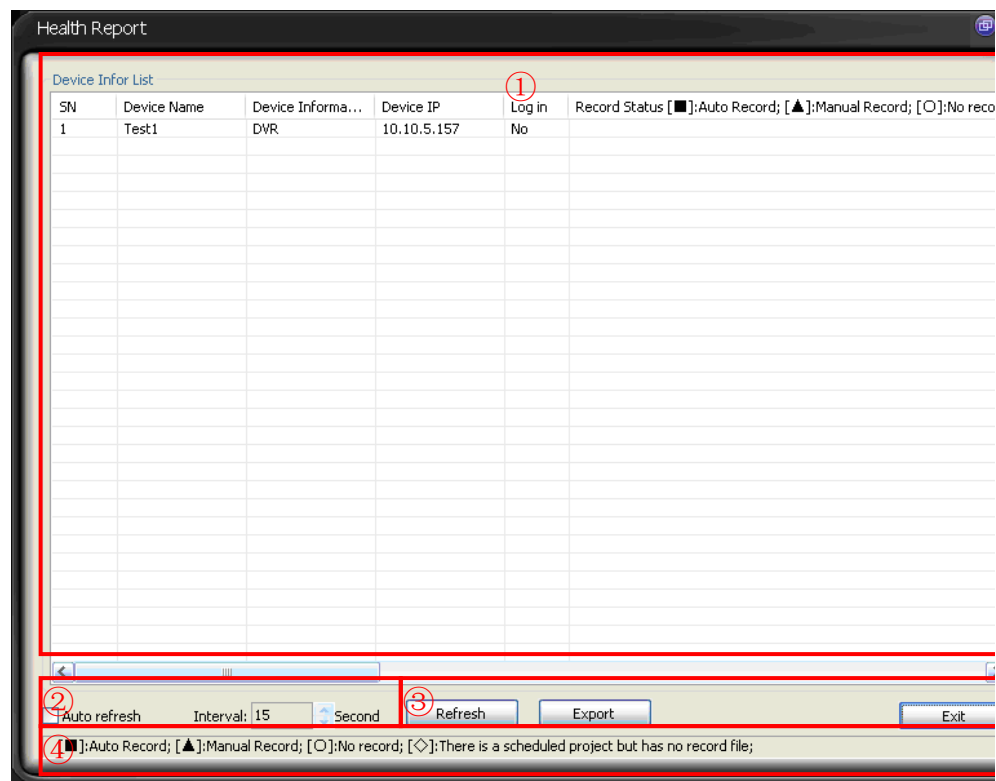
Figure 3-46 Health Report
