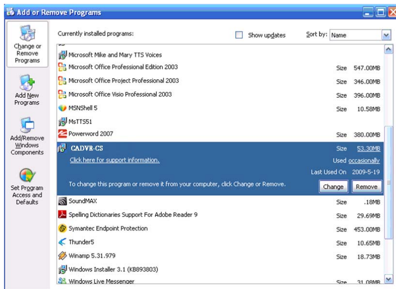
Figure 2-14 Windows Menu
