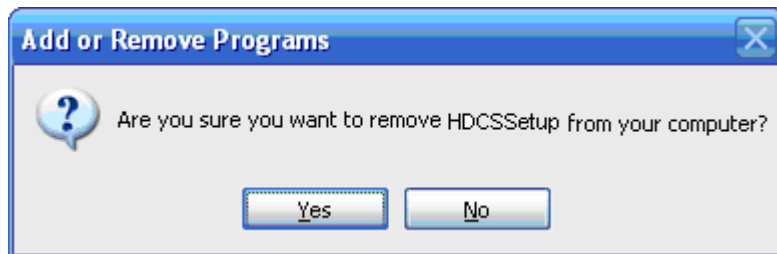
Figure 2-15 Un-installation
