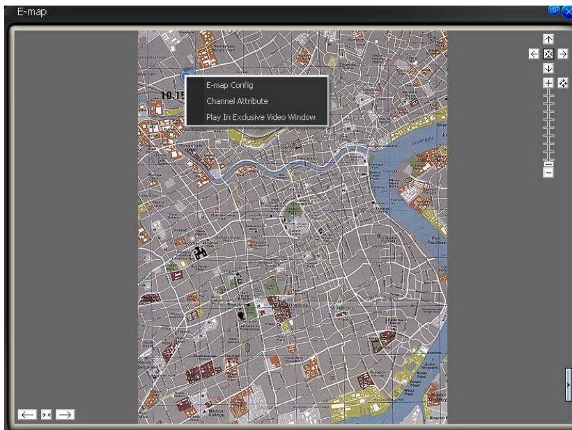
Figure 3-24 E-map Configuration 2
