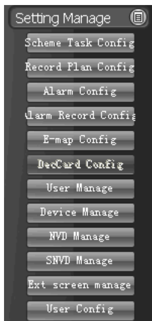
Figure 3-53 Setting Manage
