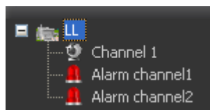
Figure 3-21 E-map organization
