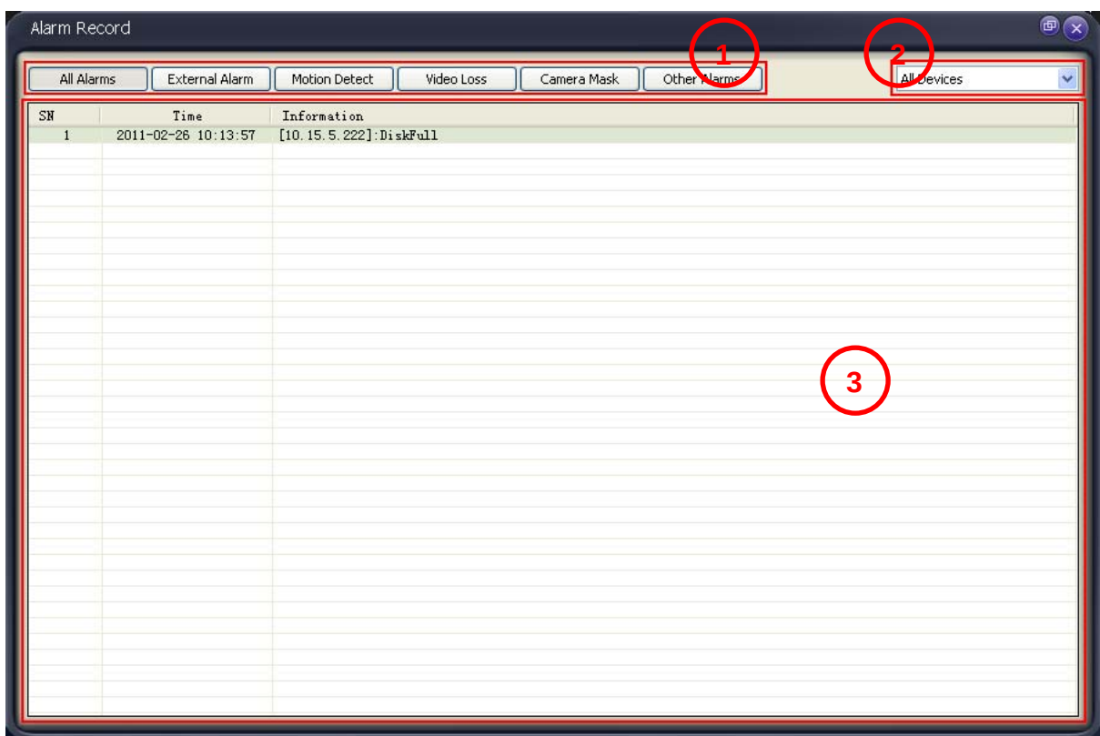
Figure 3-11 Alarm Record
