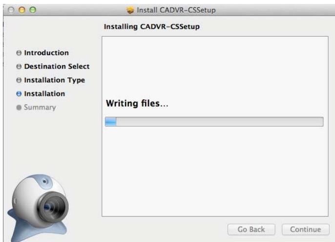
Figure 2-11 MAC Installation 4
