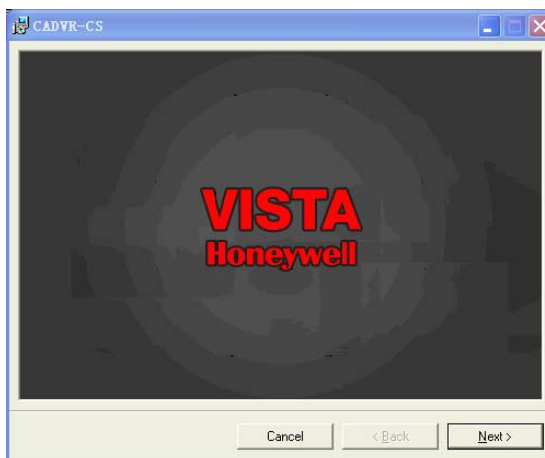
Figure 2-1 Installation 1
