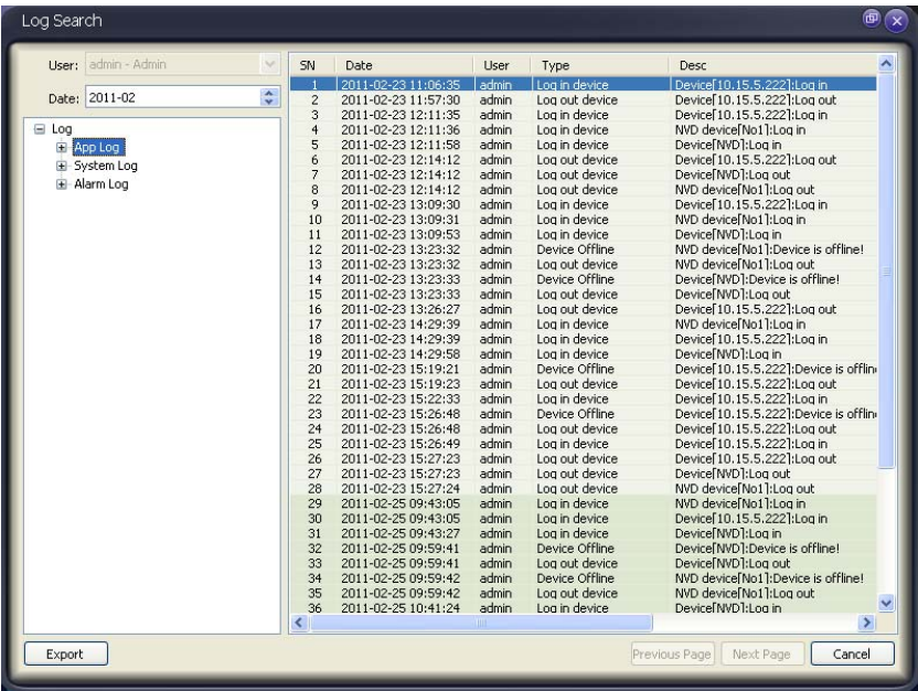
Figure 3-47 Log Search
