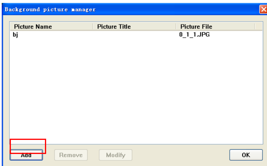
Figure 3-67 Add E-map 6-1
