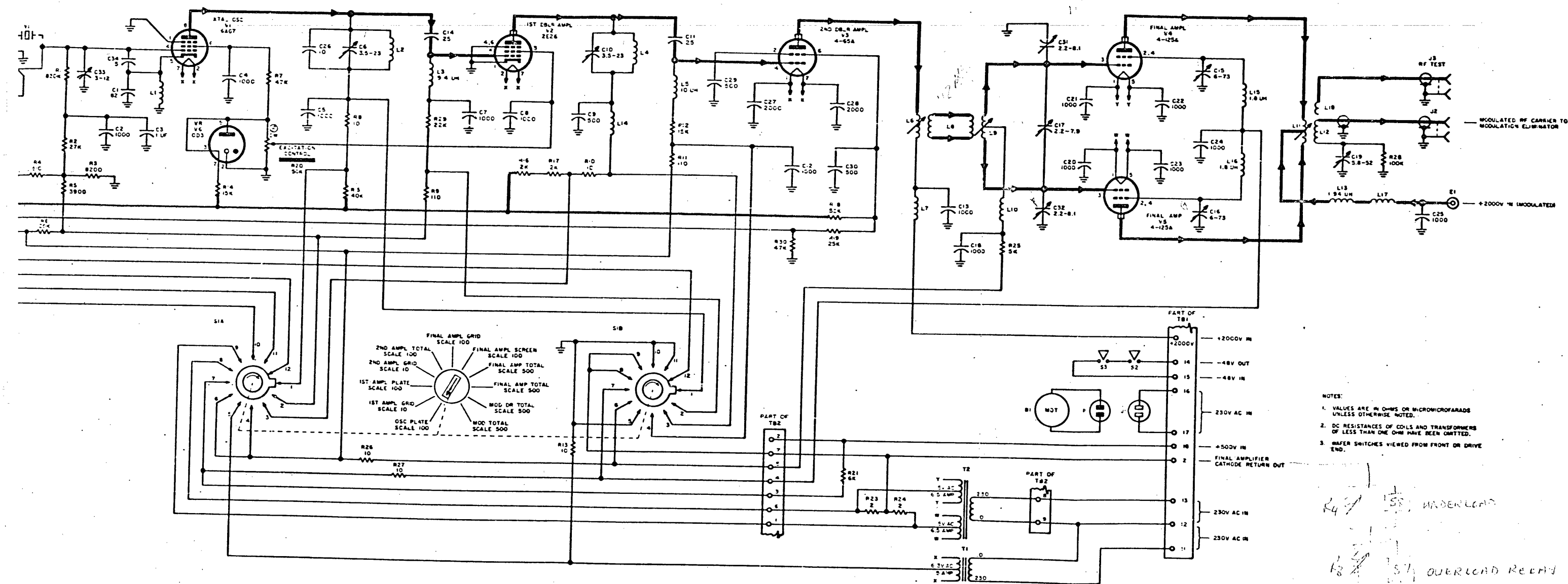
Figure 7-11. VHF RF Unit, Schematic Diagram
