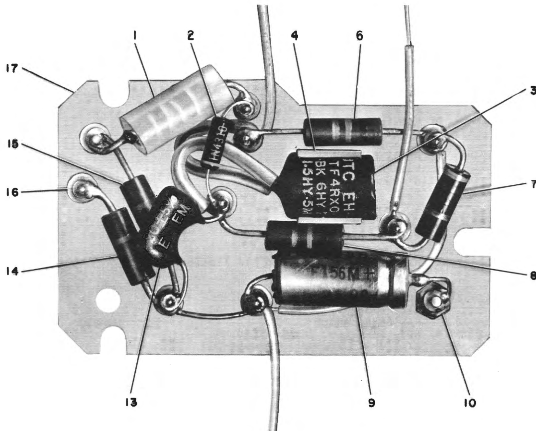
Figure 6-6. RF Detector
