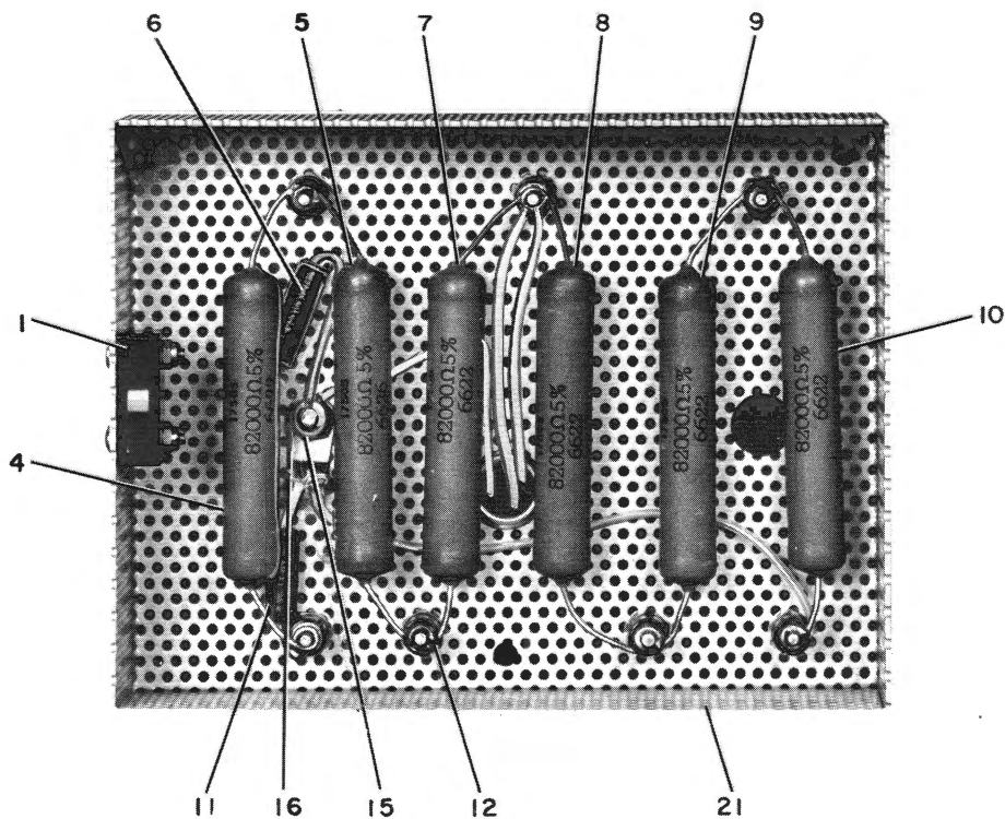
Figure 6-10. Resistor Assembly
