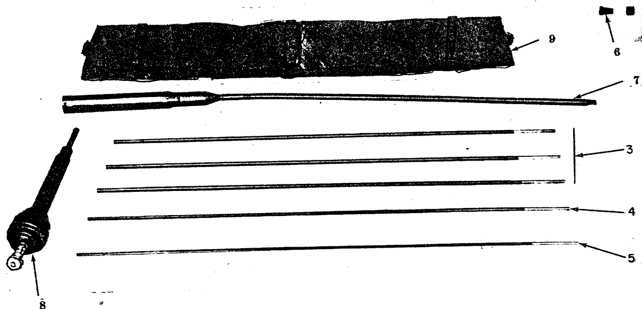
ANTENNA AS-1320
