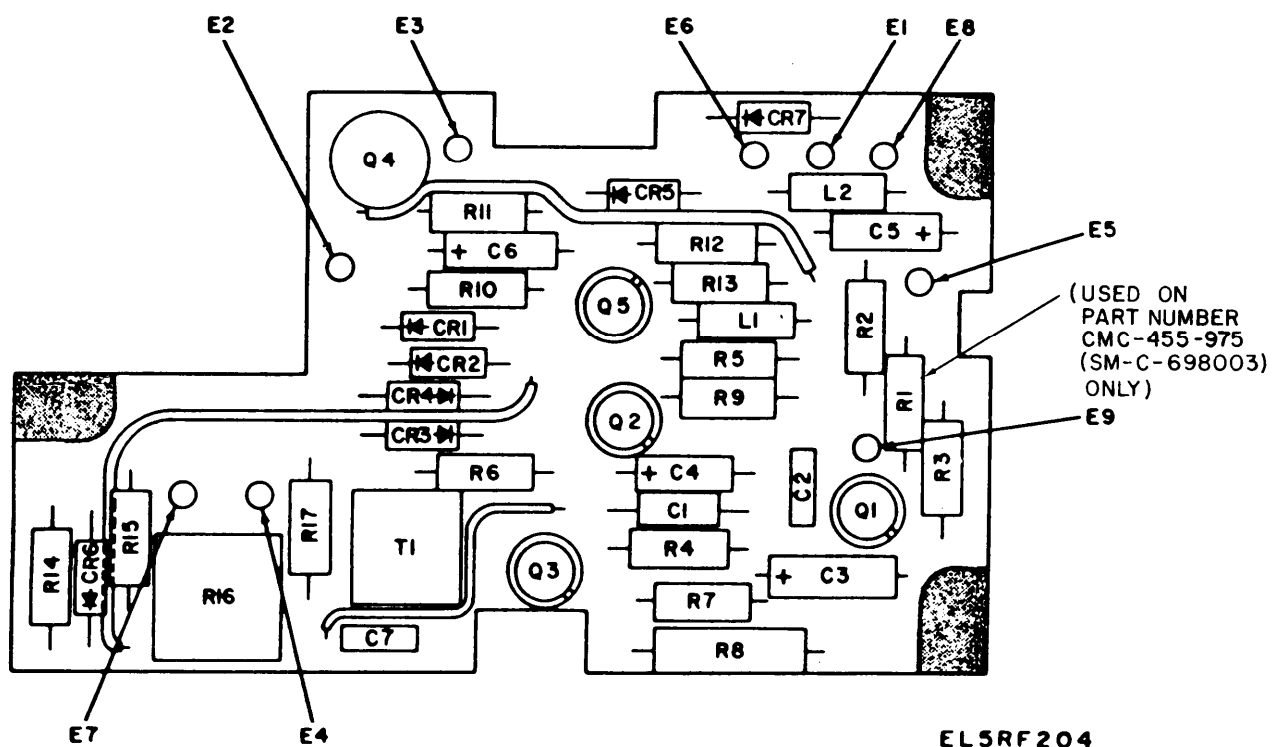
Figure 3-61. Alarm Control 1RE1AR1A3, Parts Location.
