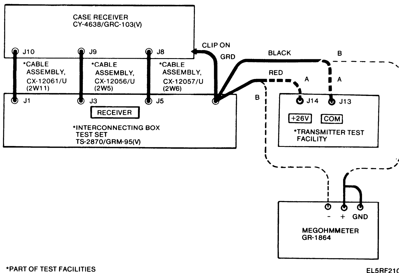
Figure 3-72. Receiver Case Continuity Check, Test Setup.
