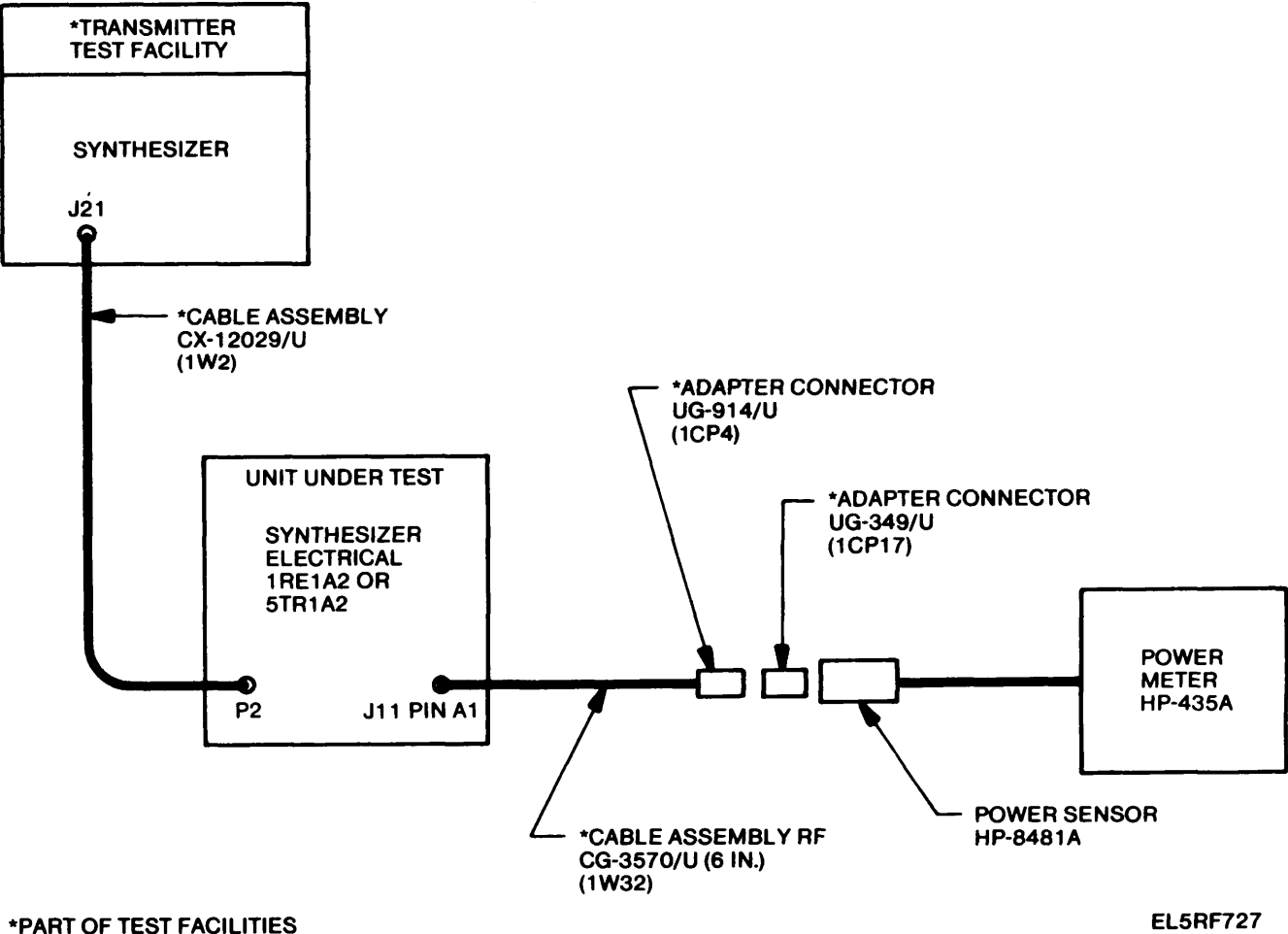
Figure 3-85. Electrical Frequency Synthesizer, Power Output, Test Setup.
