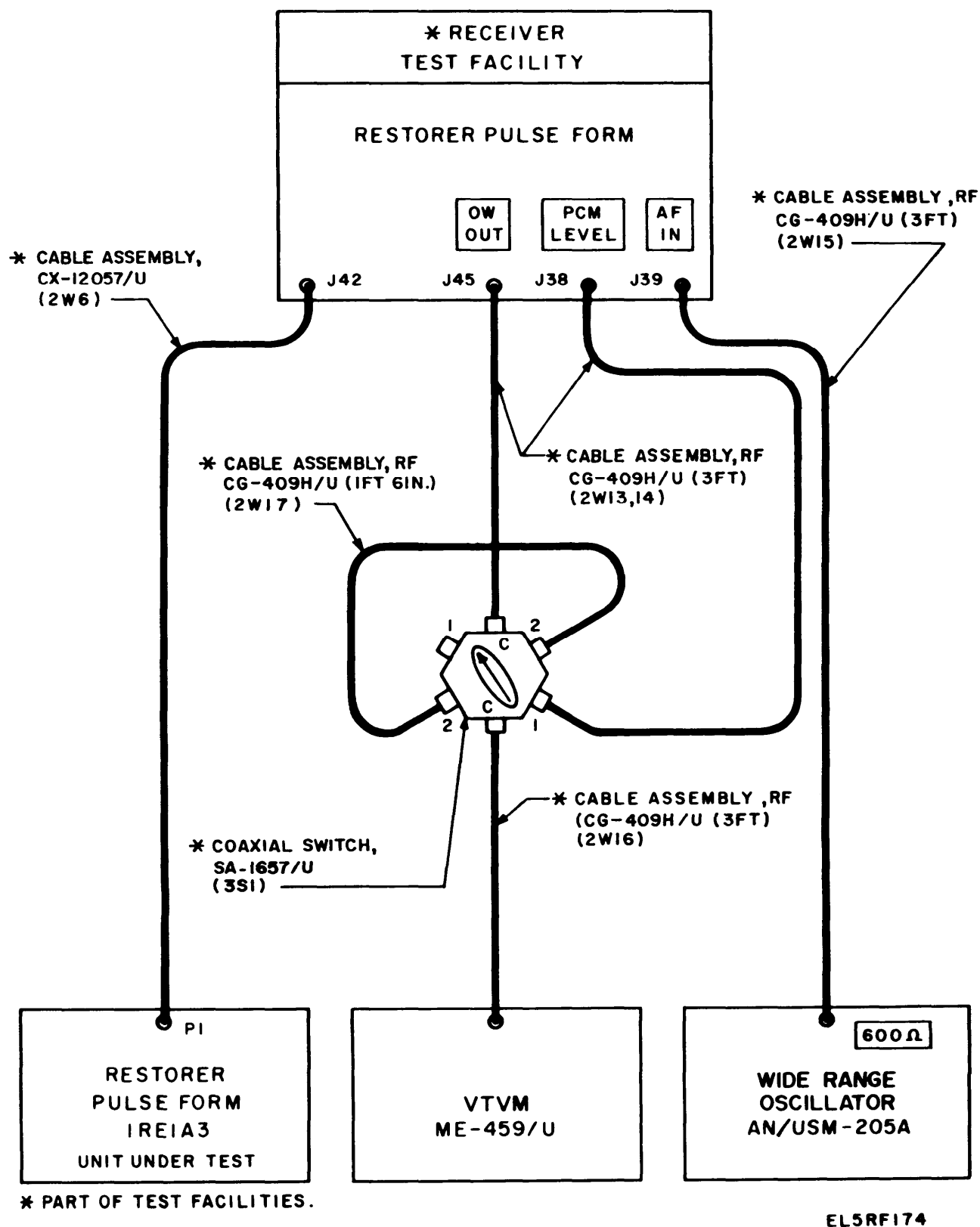
Figure 3-18. Pulse Form Restorer 1RE1A3, (SM-D-698146) Order Wire Gain and Frequency Response Check Test Setup.
