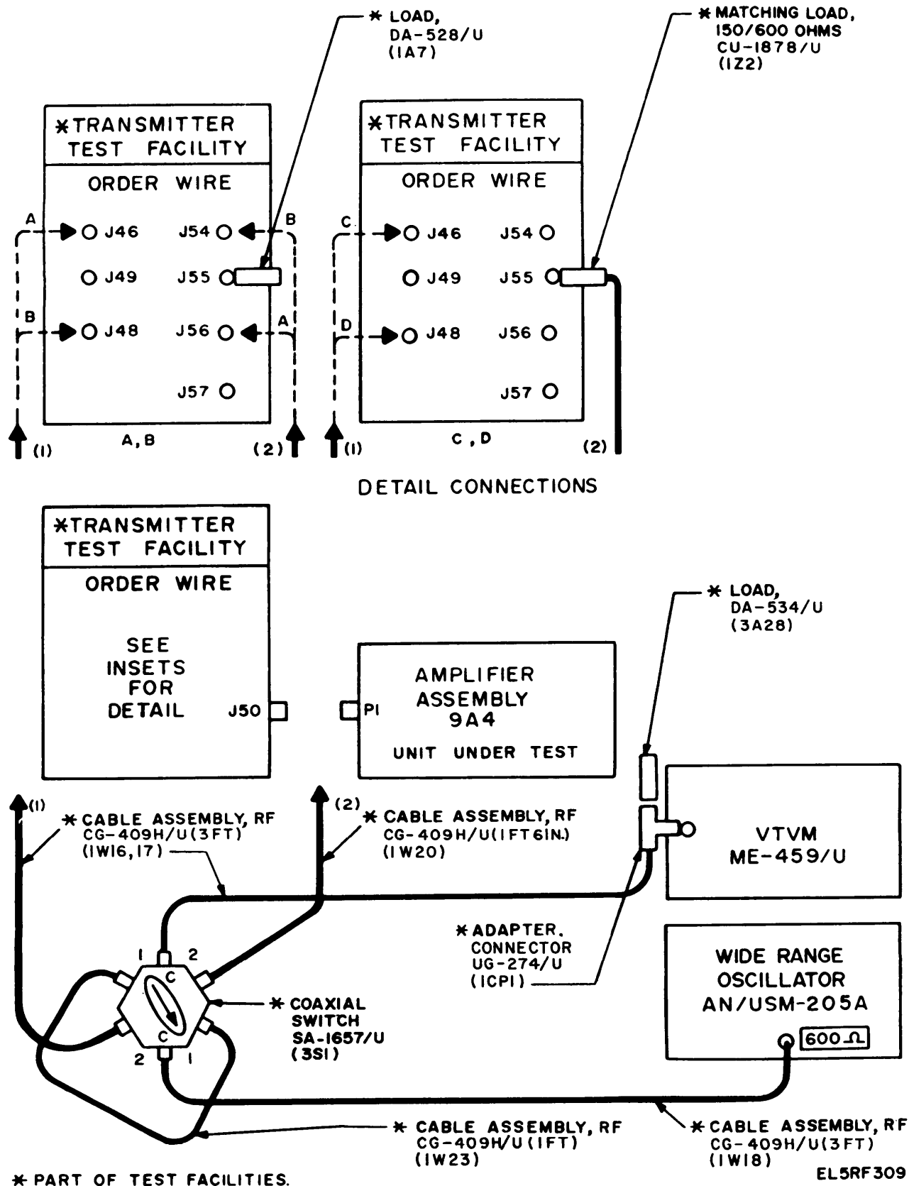
Figure 3-143. Order Wire Crosstalk Measurement, Test Setup.
