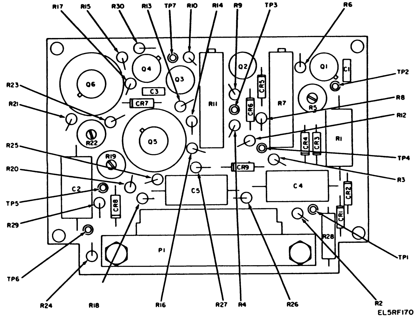
Figure 3-12. Voltage Regulator Amplifier 1RE1RS1AR1AR1, Parts Location.
