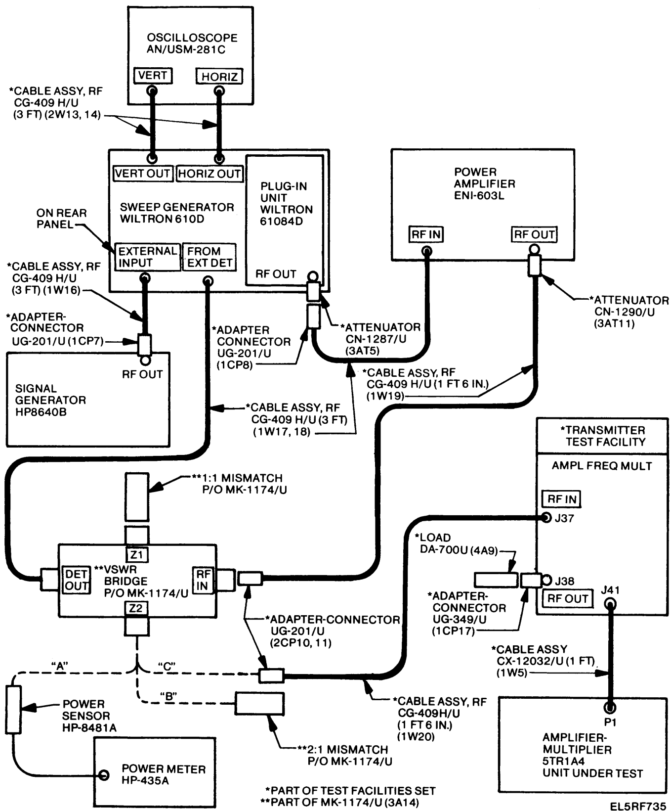
Figure 3-102. Amplifier-Frequency Multiplier 5TR1A4 VSWR Test Setup.
