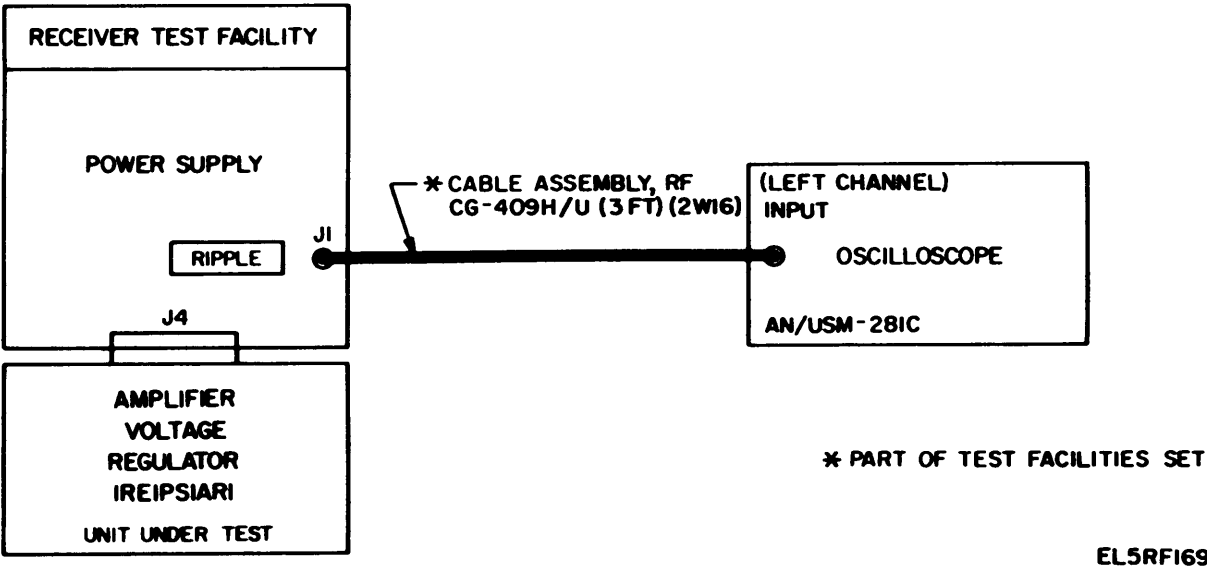
Figure 3-11. Voltage Regulator Amplifier 1RE1PS1AR1, Test Setup.
