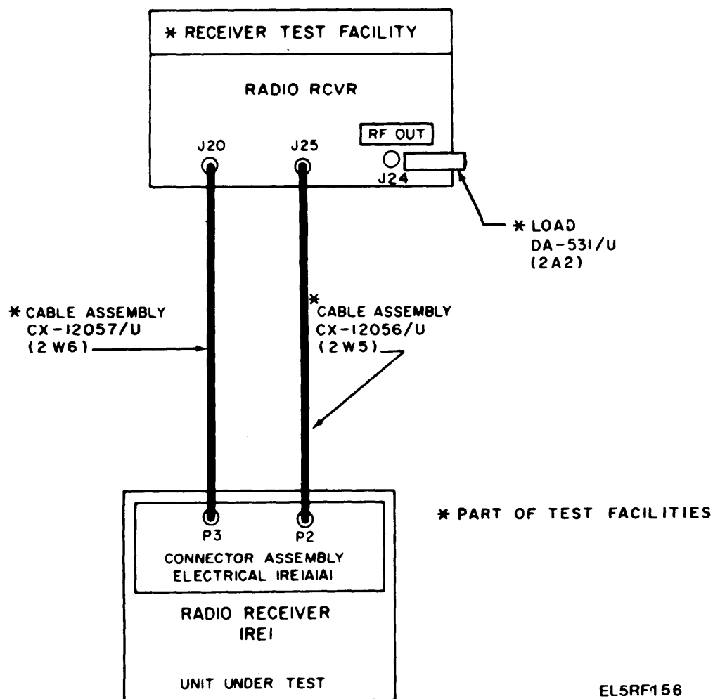
Figure 3-1. Receiver Fixed Head, Operational Check Test Setup.
