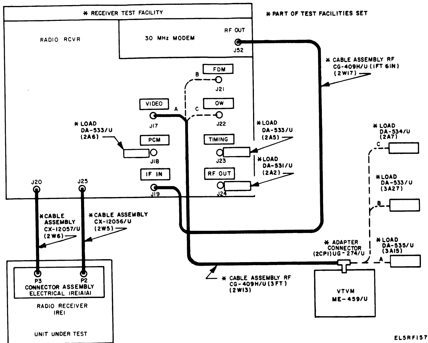
Figure 3-2. Receiver Fixed Head, Video Level, Metering and Wideband Noise Check, Test Setup.
