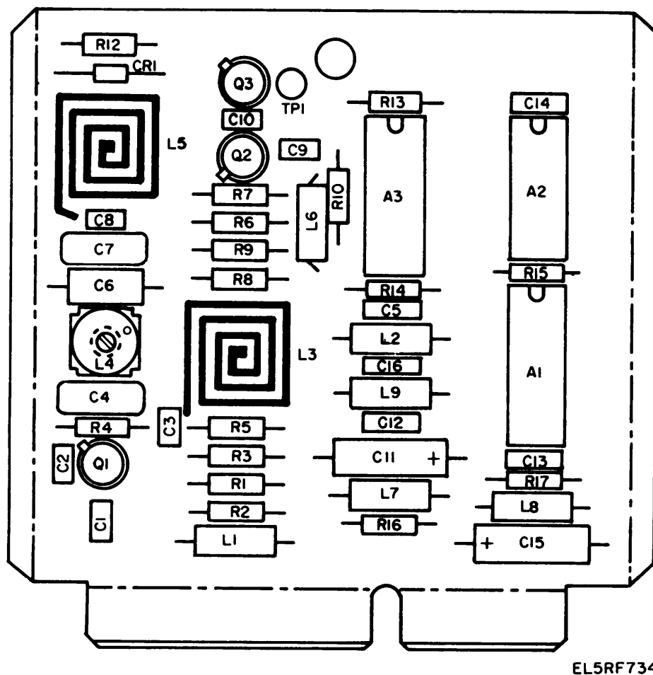
Figure 3-96. Frequency Divider 1RE1A2A14 or 5TR1A2A14, Parts Location
