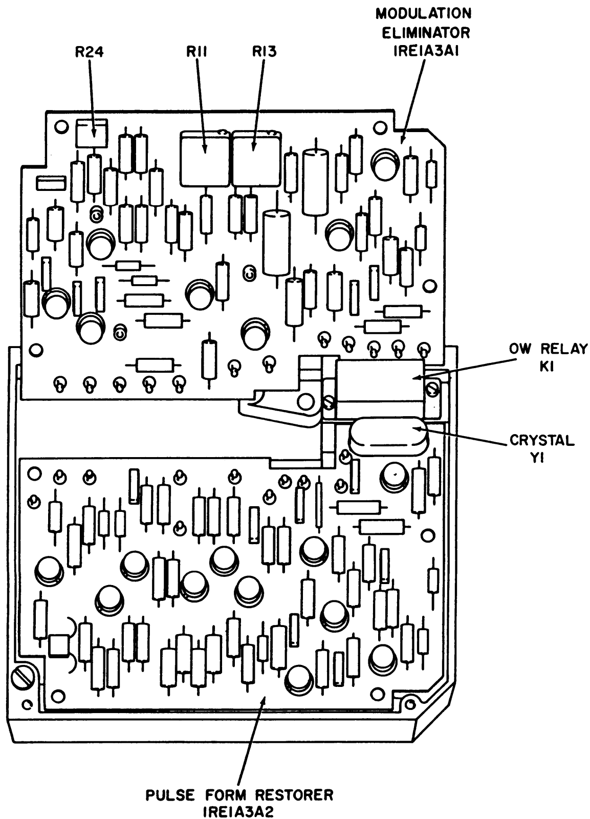
Figure 3-23. Pulse Form Restorer 1RE1A3 (SM-D-698146), Opened Showing Pulse Form Restorer 1RE1A3A2.
