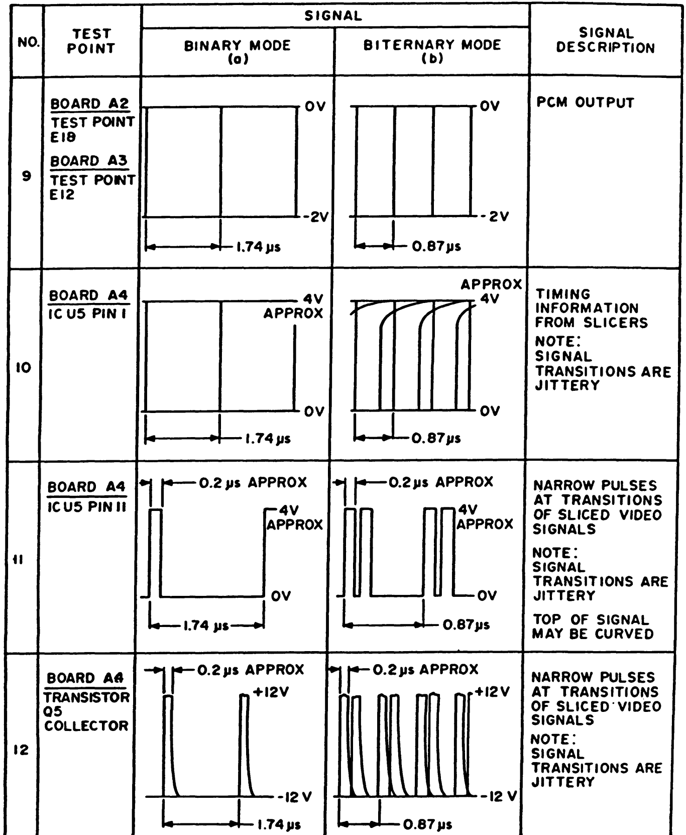
Figure 3-35. Waveform Diagrams for Pulse Form Restorer 1RE1A3 (SM-D-990510) (Sheet 3).
