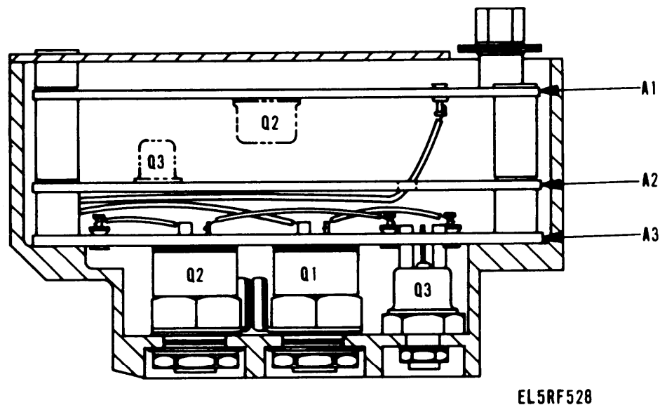
Figure 3-129. Control Monitor Temperature Sensor, 5A2A2, Parts Location
