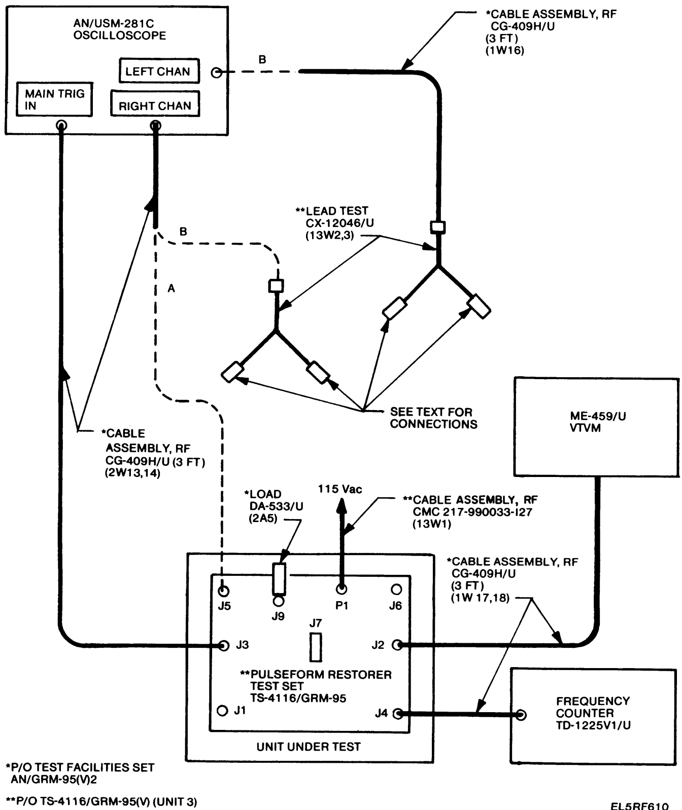
Figure 3-24. Pulse Form Restorer 1RE1A3 (SM-D-990510), Timing Phase Adjustment, Test Setup.
