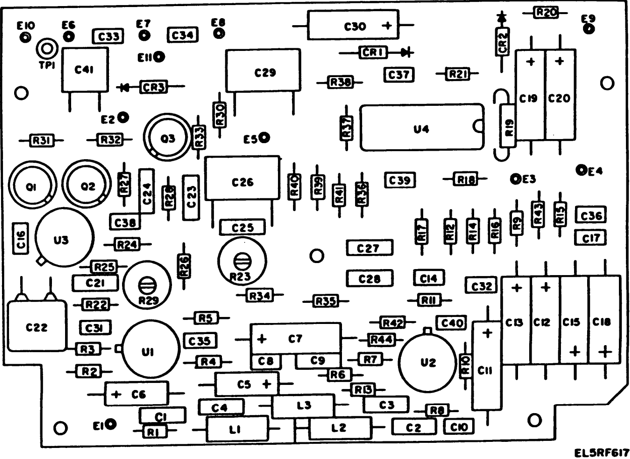
Figure 3-32. Pulse Form Restorer 1RE1A3 (SM-D-990510), Modulation Eliminator Pcb 1RE1A3A1, Compment Location Diagram
