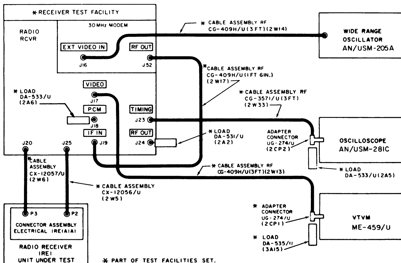
Figure 3-3. Receiver Fired Head PCM Regeneration Timing, and PCM Squelch Check Test Setup
