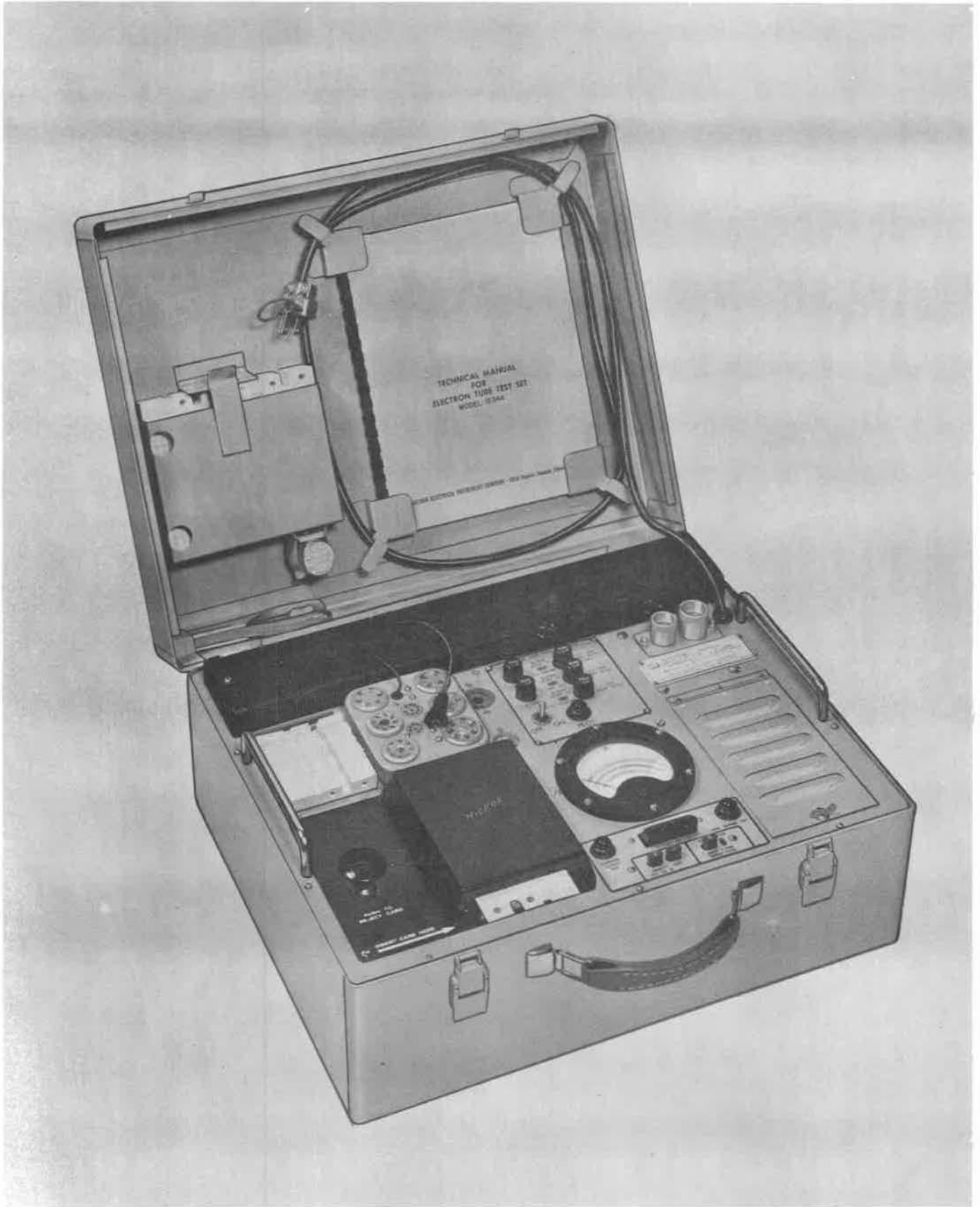
Fig. 1 Model 1234A Tube Tester
