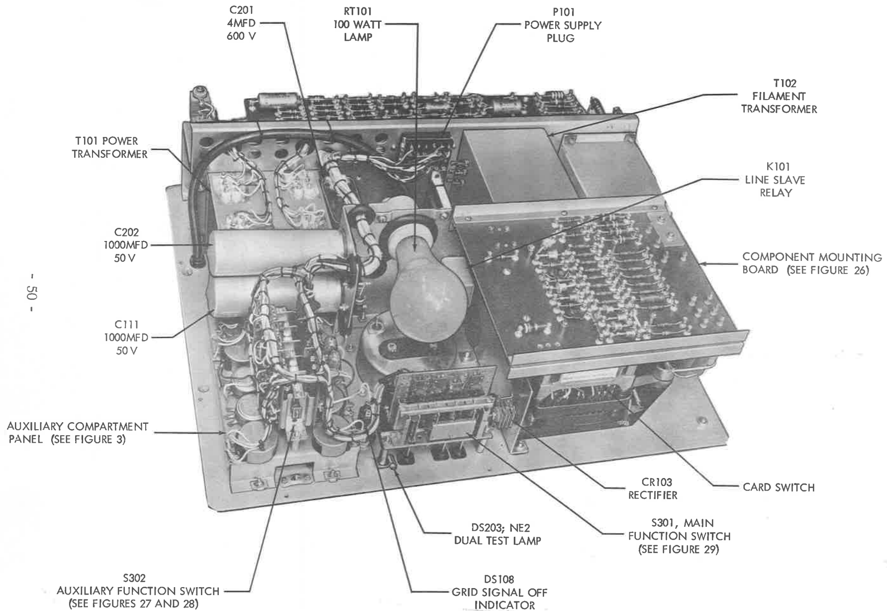
Figure 23 - Assembly Identification and Miscellaneous Parts
