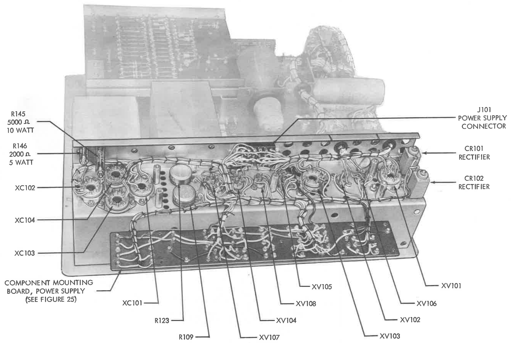
Figure 24 - Power Supply Component Location
