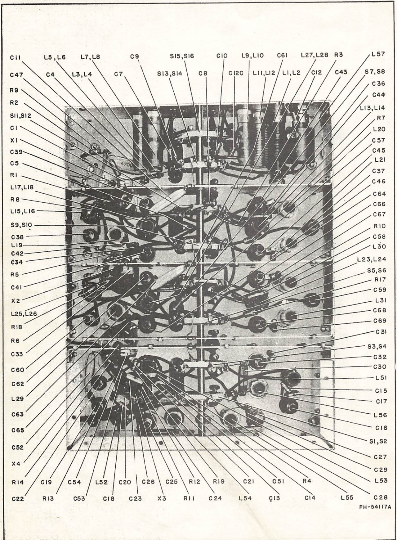
Figure 10—R-F Unit
