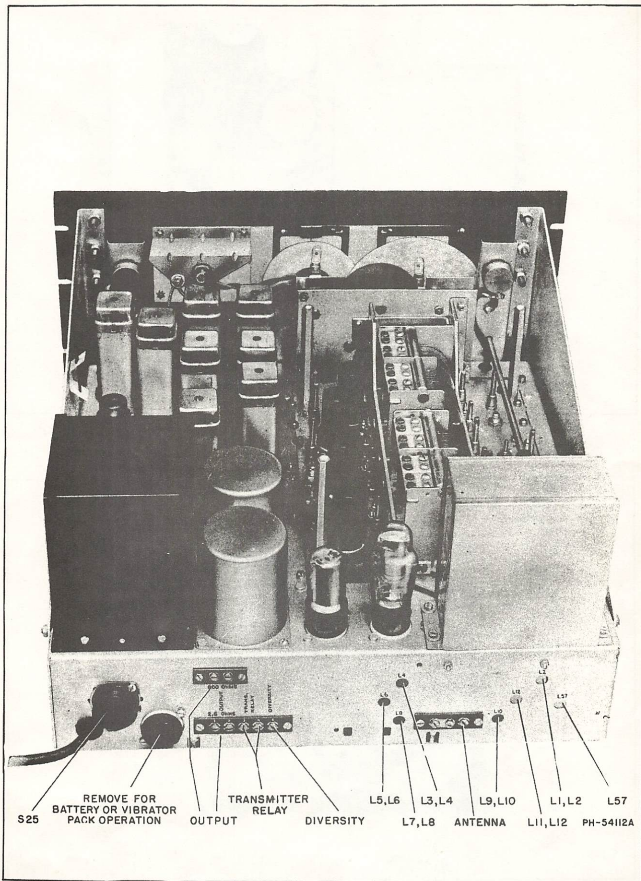
Figure 6—AR-88 Chassis
