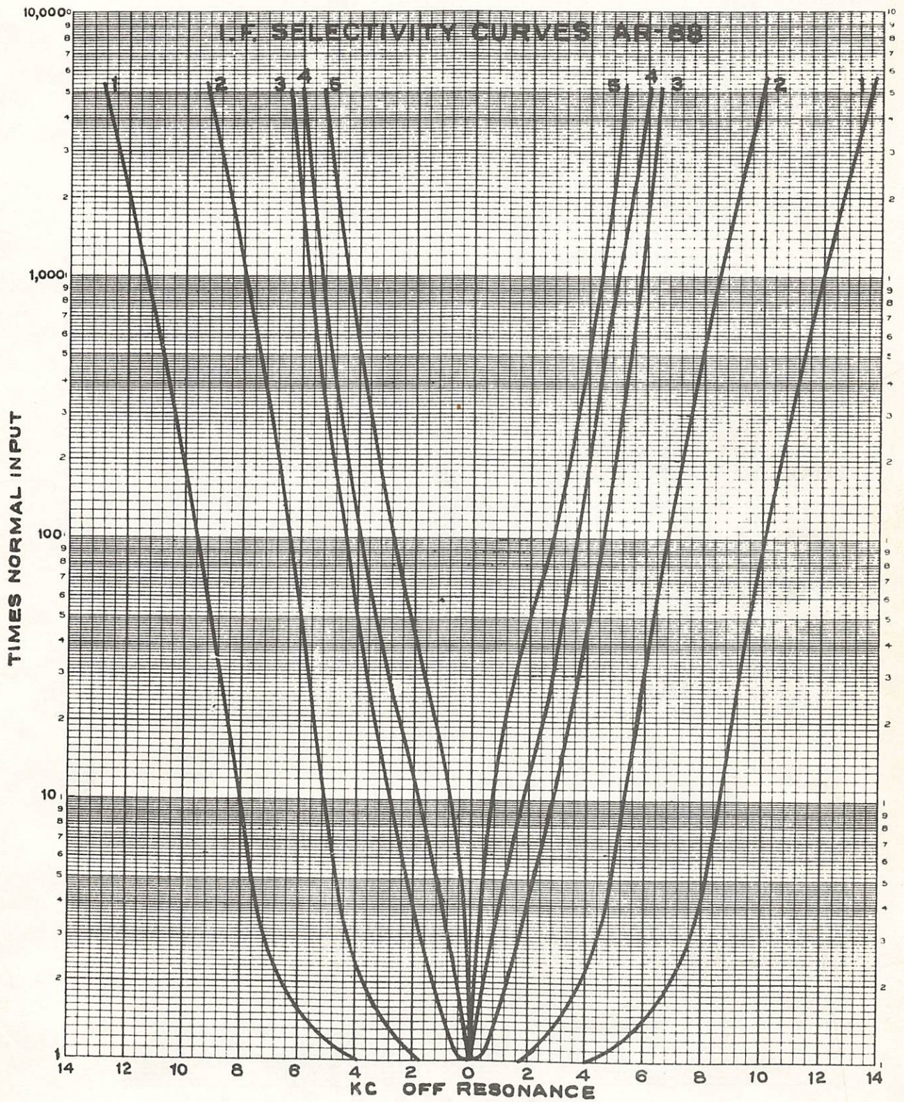
Figure 12—Selectivity Curves .
