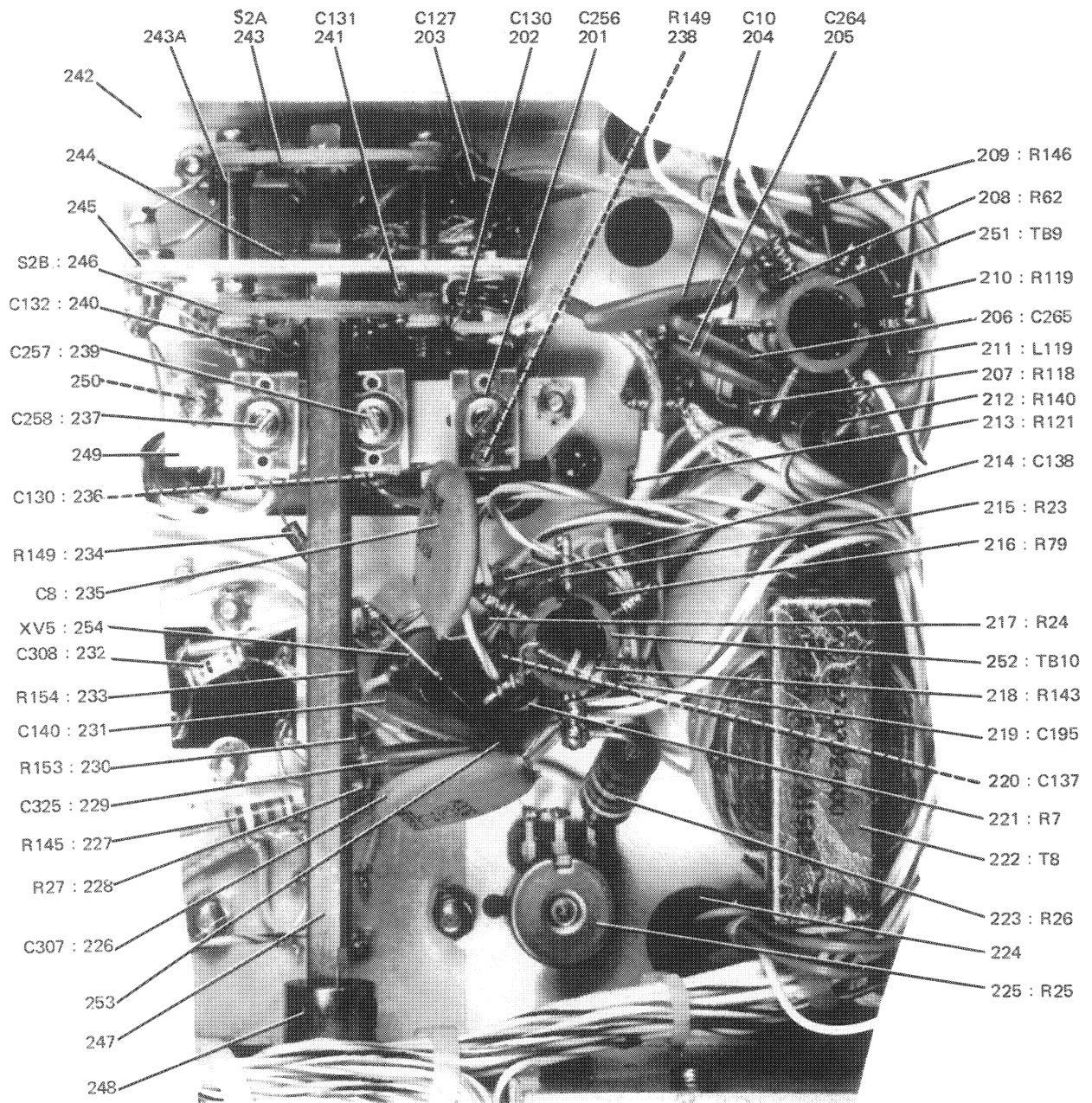
DETAIL D
