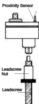
Quick release Leadscrew and Nut Assembly
