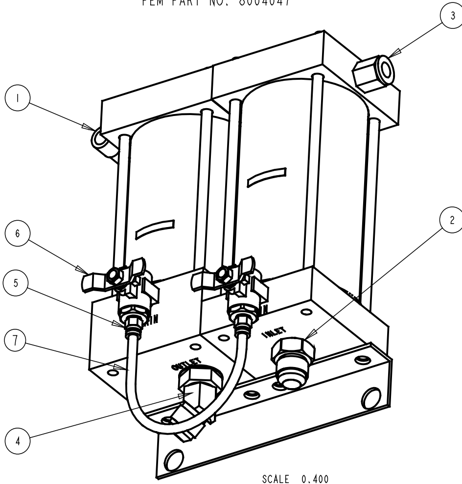
FIGURE 2.1 SERIES 2000 AIR/OIL TANKS ASSEMBLY PEM PART NO. 8004047
