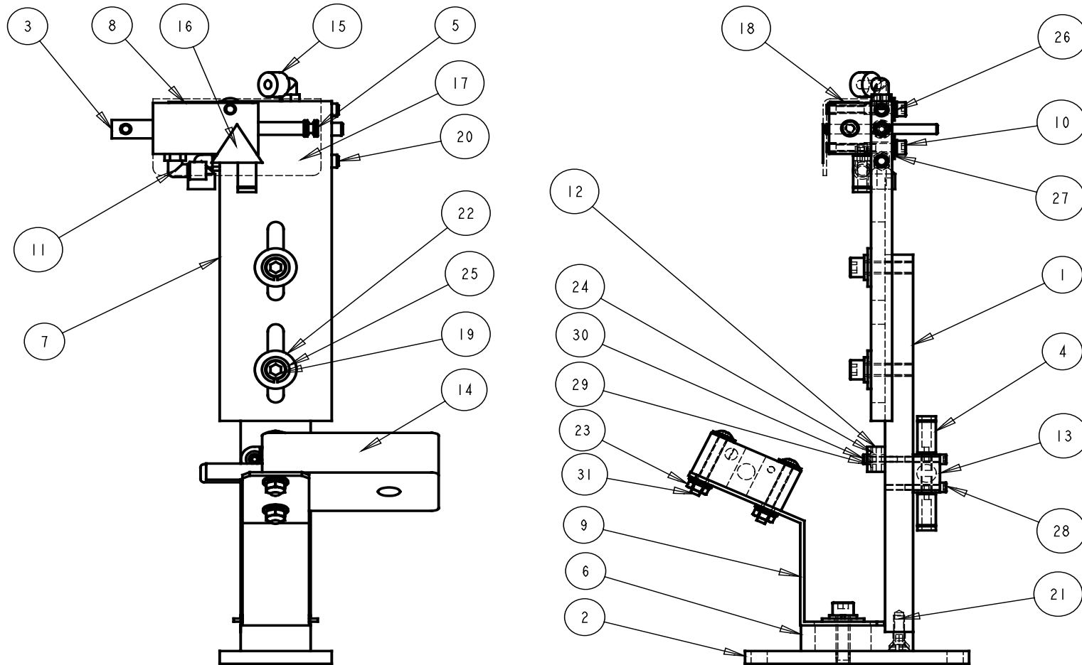
FIGURE 7.1 SERIES 2000 SHUTTLE SUPPORT ASSEMBLY PEM PART NO. 8000597 (SHOWN WITH STUD-IN-TUBE SENSOR)
