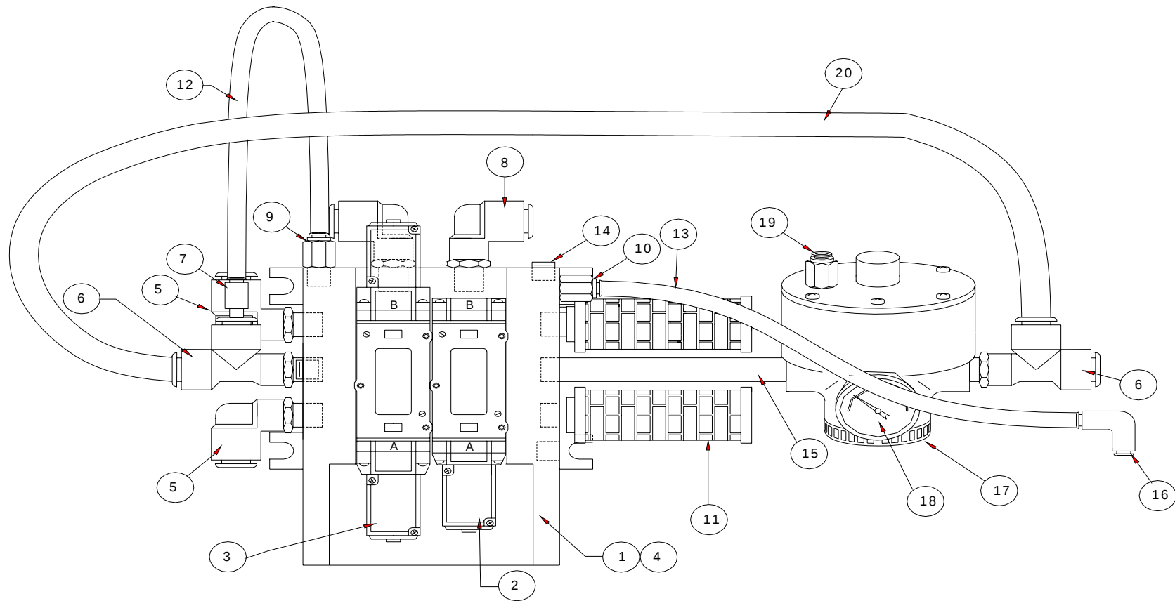
FIGURE 2.2 SERIES 2006 - RAM VALVE ASSEMBLY PEM PART NO. 8003515
