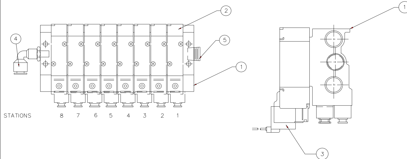
FIGURE 8.1 SERIES 2000 – 8-STATION MANIFOLD ASSEMBLY – VER 3 PEM PART NO. 8003054
