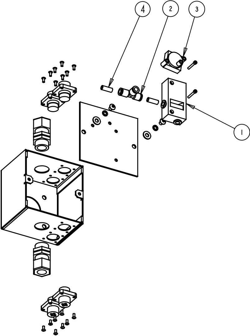
FIGURE 4.1 SERIES 2000 DISTRIBUTION BOX ASSEMBLY PEM PART NO. 8003551
