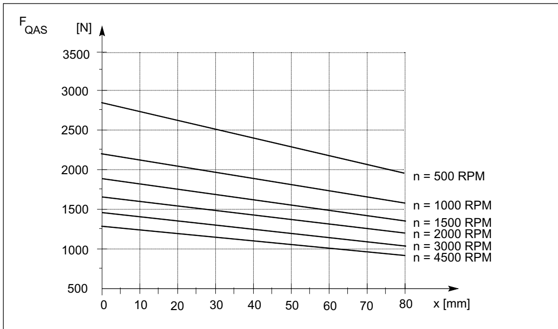
Fig. 3-38 Cantilever force F_Q at a distance x from the shaft shoulder for a nominal bearing lifetime of 20,000 h
