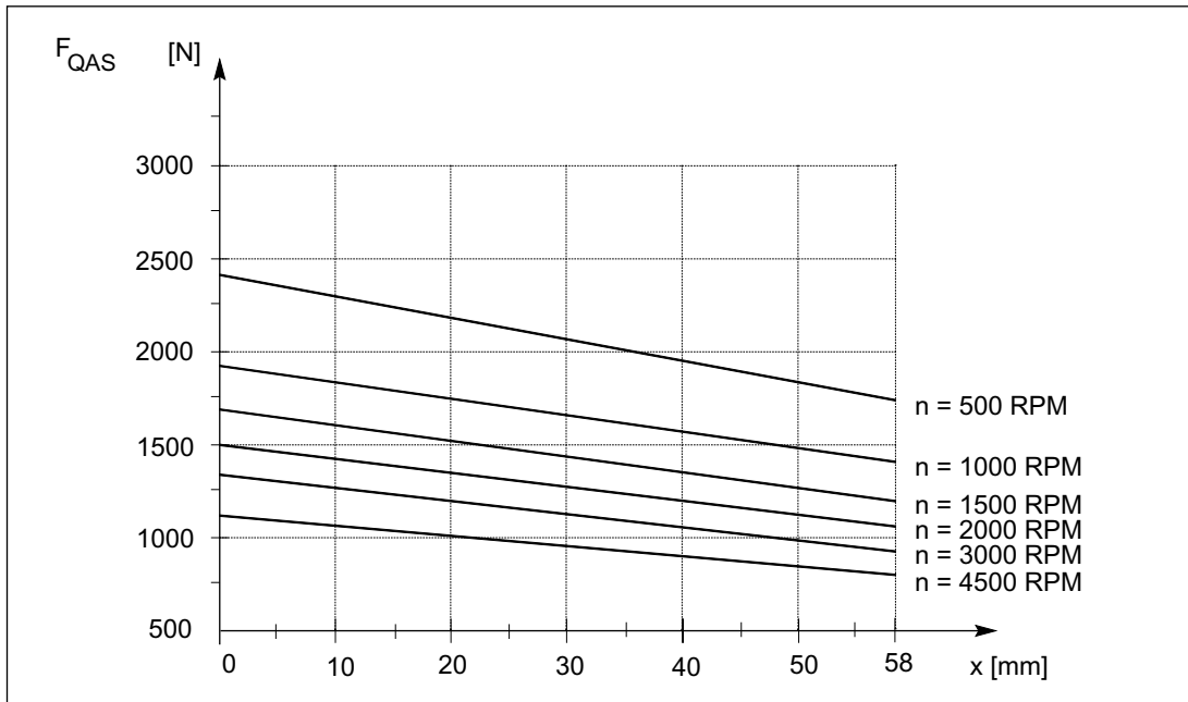
Fig. 3-37 Cantilever force F_Q at a distance x from the shaft shoulder for a nominal bearing lifetime of 20,000 h
