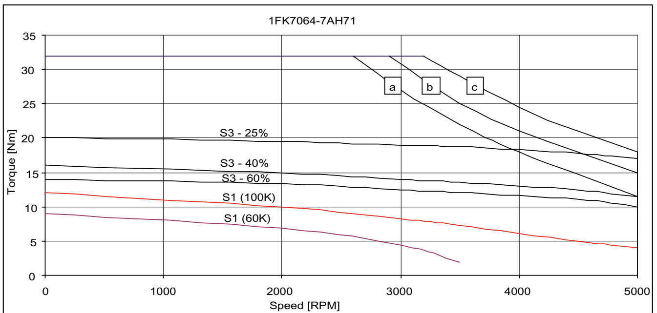
Fig. 3-28 Speed-torque diagram 1FK7064-7AH71 HD
