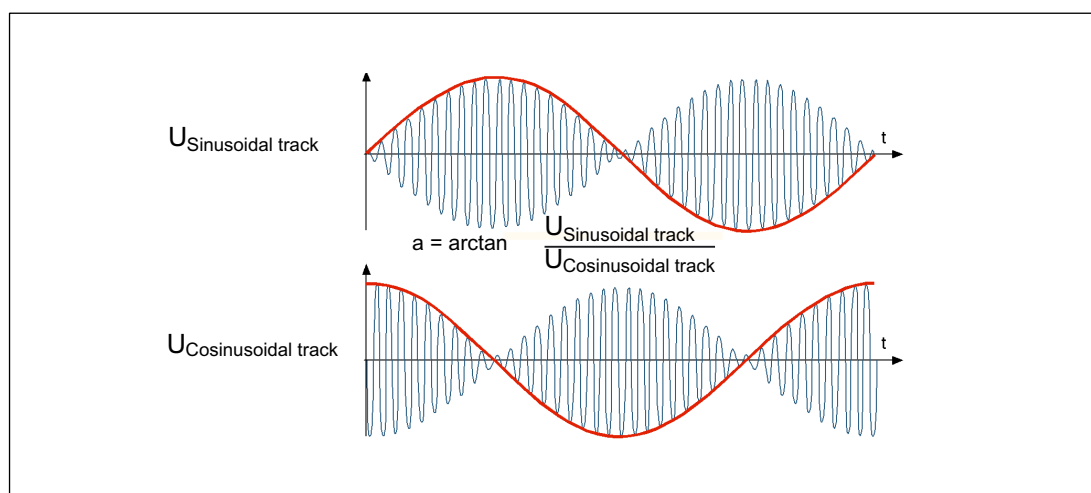
Fig. 4-4 Output signals, resolver
