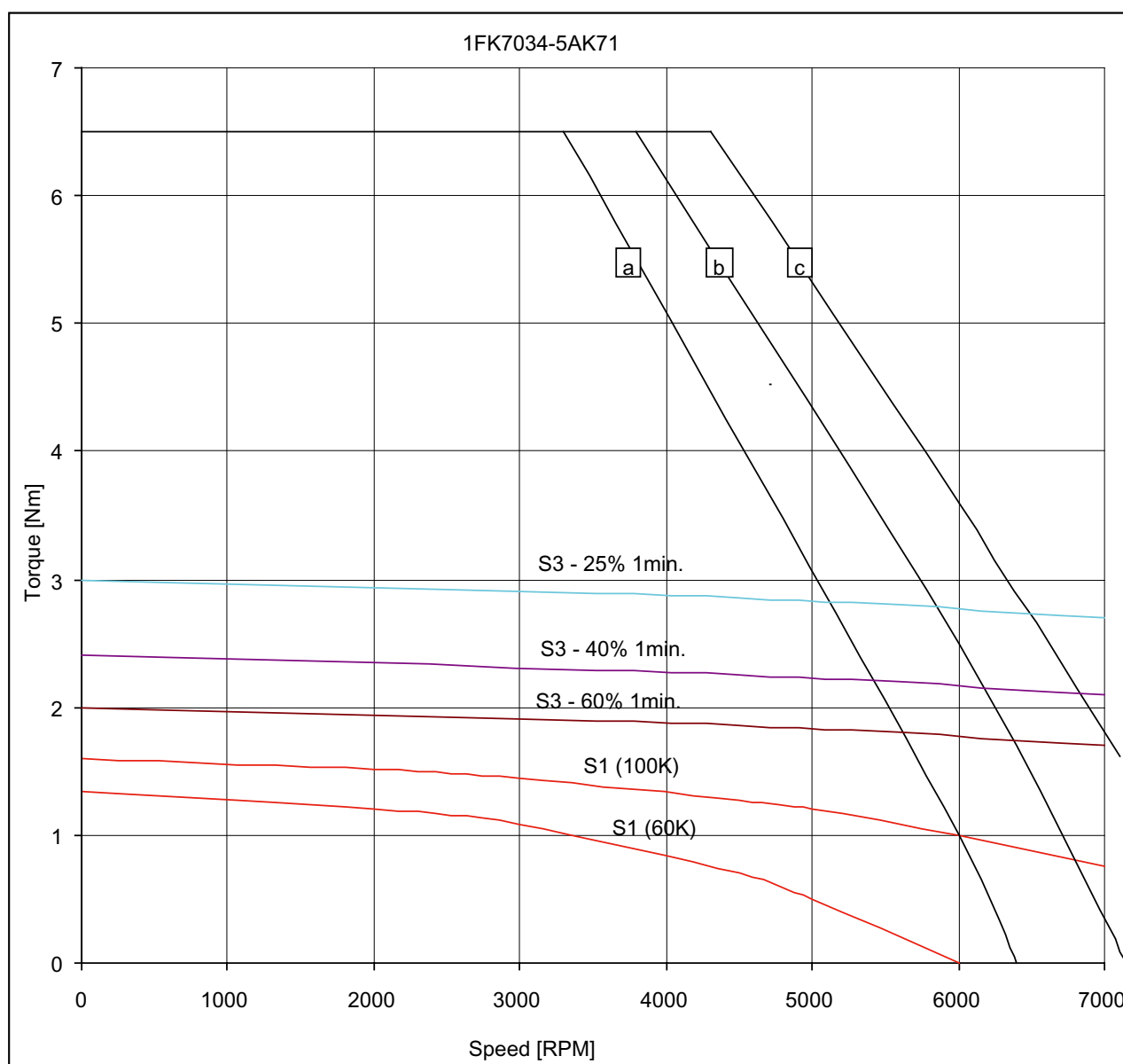
Fig. 3-3 Speed-torque diagram 1FK7034-5AK7 CT
