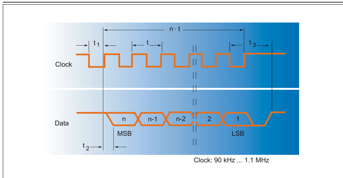
Fig. 4-3 Output signals, absolute encoders
