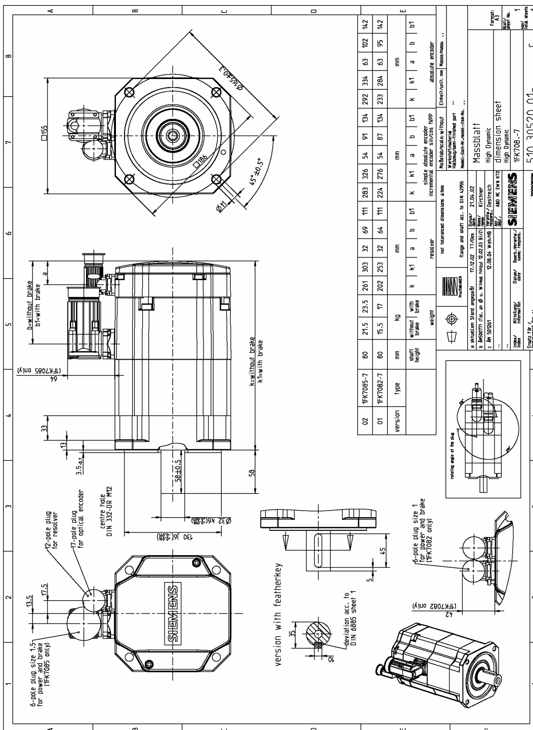
Fig. 6-12 1FK7082-7, 1FK7085-7
