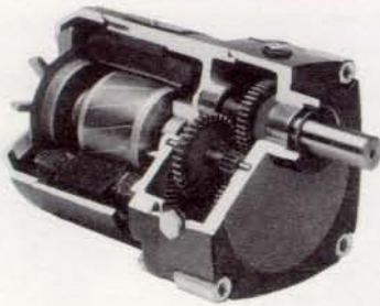
"N-1D" Gearmotor
