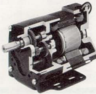
"30R-D" Gearmotor
