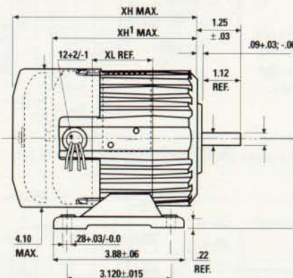
Dimensions (inches)
