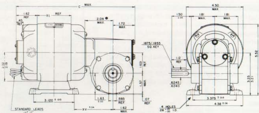
"N-3RH" Gearmotor
