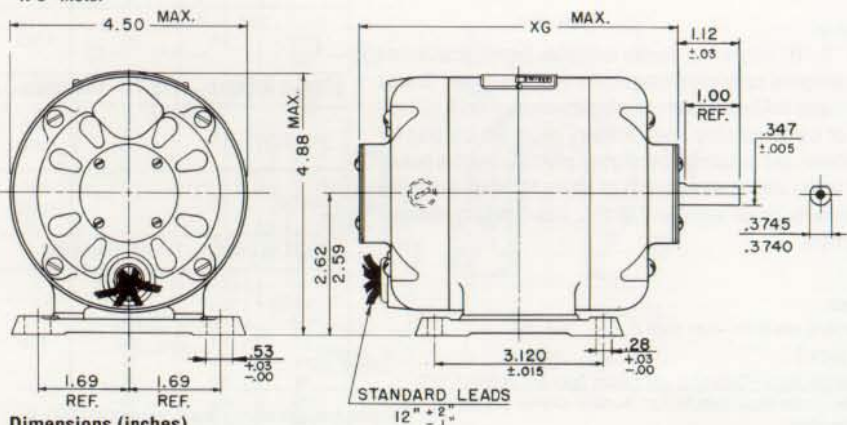
Dimensions (inches)
