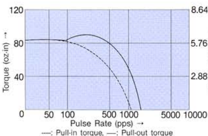
PJ80B1 Torque Characteristics (Chopper Drive)
