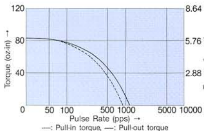
PJ80B1 Torque Characteristics (L/5.2R)
