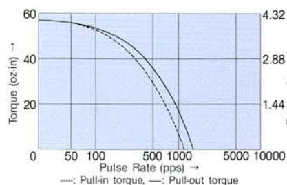
PJ55B1 Torque Characteristics (L/5.3R)
