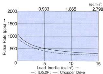
PJ80B1 Starting Characteristics
