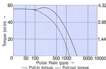
PJ55B1 Torque Characteristics (Chopper Drive)
