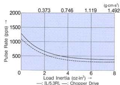
PJ80B1 Starting Characteristics
