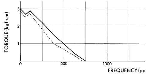
SST55D2040 DRIVER : TYPE A (C = 1 \mu F, R = 0) VOLTAGE : V w = 24 V EXCITING MODE = 2 Phase INERTIAL LOAD : 100 g-cm 2
