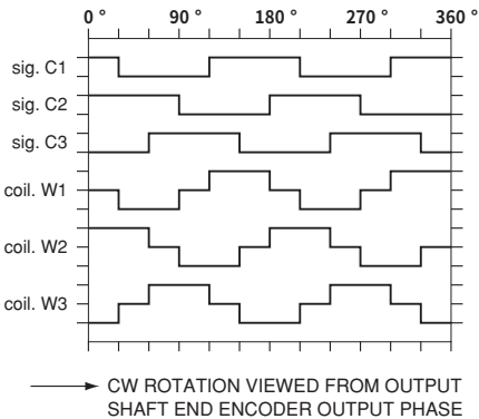
TIMING DIAGRAM
