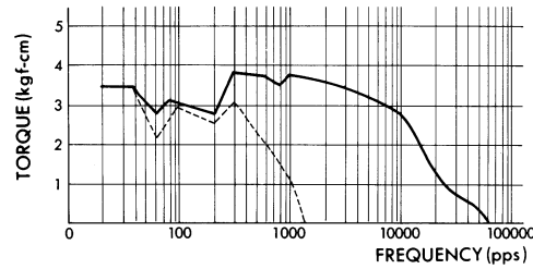
SST55D2010 DRIVER : SDU2401 CURRENT = 3.2 A/Phase EXCITING MODE = 2 Phase INERTIAL LOAD : 100 g-cm 2
