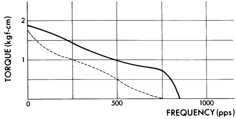
SST55D1040 DRIVER : TYPE A (C = 1 \mu F, R = 0) VOLTAGE : V w = 24 V EXCITING MODE = 2 Phase INERTIAL LOAD : 100 g-cm 2
