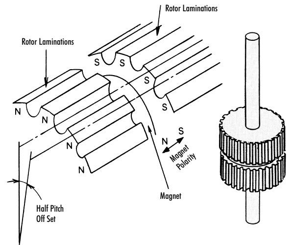
Fig. 5-2 Rotor Construction
