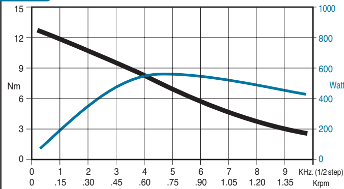
SANYO 103 8960 6551 - parallel bipolar connection RTA GMD03 drive
