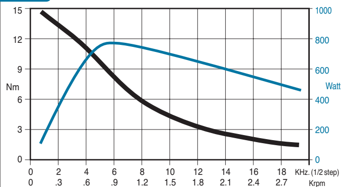
SANYO 103 8960 6551 - parallel bipolar connection RTA GMD04 drive
