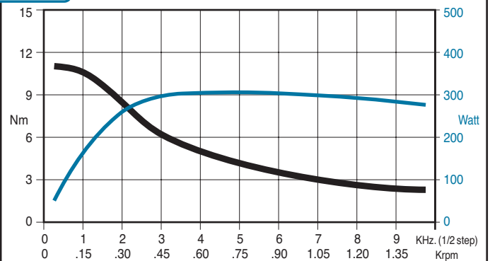
SANYO 103 8932 6451 - series bipolar connection RTA GMD04 drive
