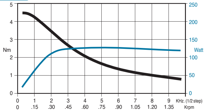
SANYO 103 845 6741 - series bipolar connection RTA GMD02 drive
