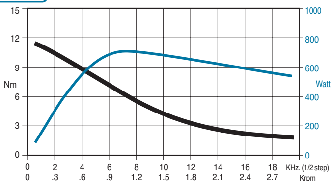
SANYO 103 8932 6451 - parallel bipolar connection RTA GMD04 drive
