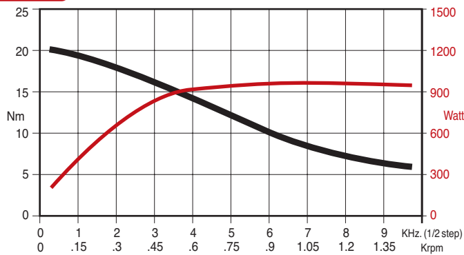
SANYO 103 H89223 6641 - bipolar connection RTA GMD04 drive
