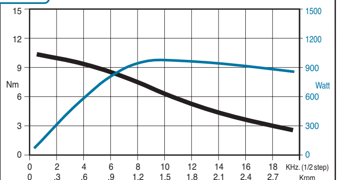
SANYO 103 8932 6451 - parallel bipolar connection RTA GMD06 drive
