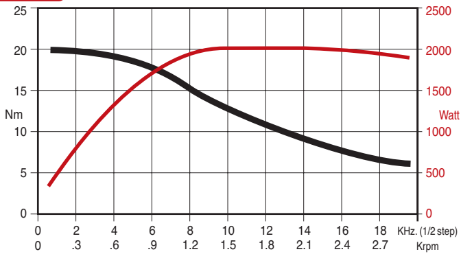
SANYO 103 H89223 6641 - bipolar connection RTA BCW02 drive
