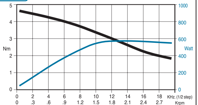
SANYO 103 845 6741 - parallel bipolar connection RTA GMD06 drive
