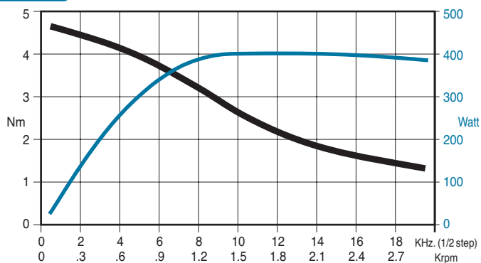
SANYO 103 845 6741 - parallel bipolar connection RTA GMD04 drive
