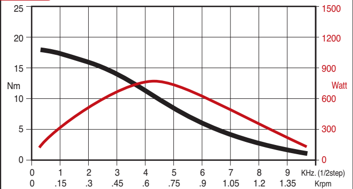
SANYO 103 H89223 6641 - bipolar connection RTA GMD03 drive
