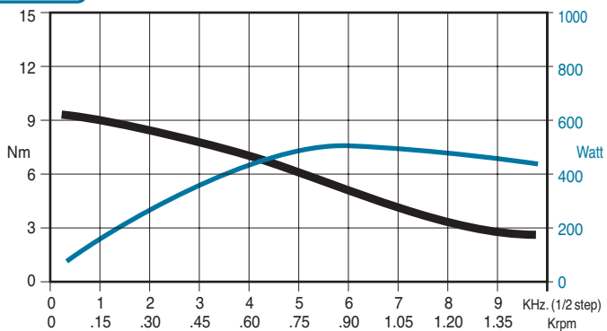
SANYO 103 8932 6451 - parallel bipolar connection RTA GMD03 drive
