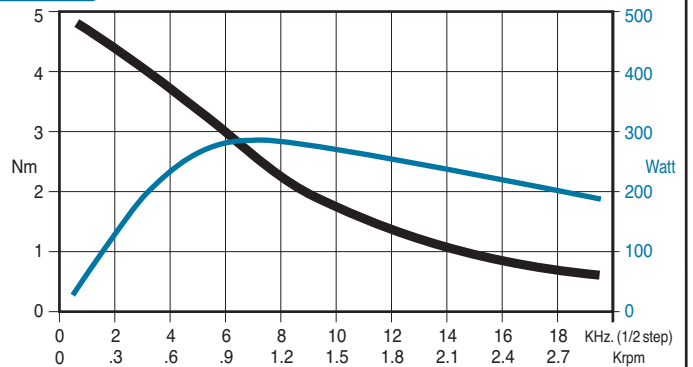
SANYO 103 845 6741 - parallel bipolar connection RTA GMD03 drive
