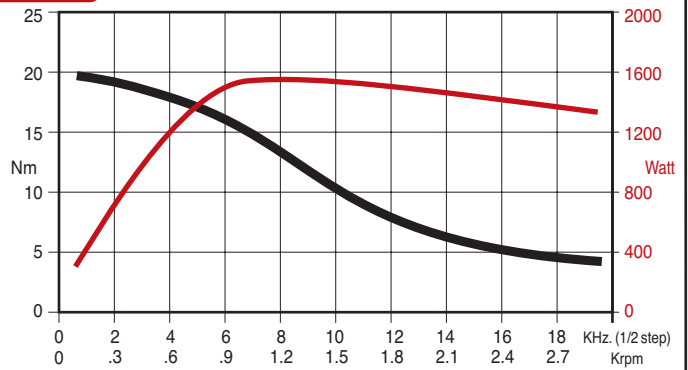
SANYO 103 H89223 6641 - bipolar connection RTA GMD06 drive
