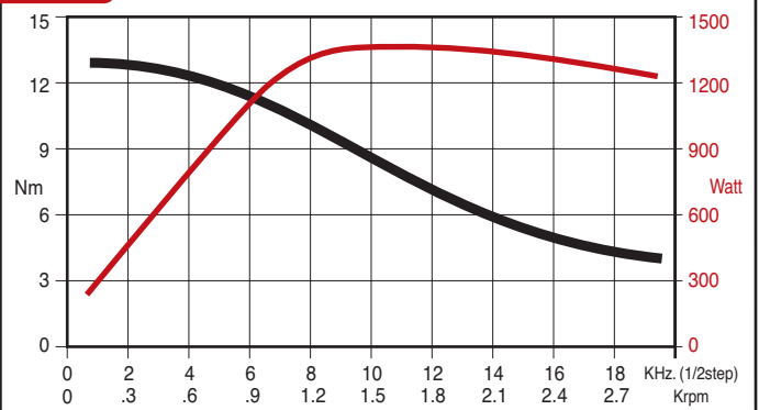
SANYO 103 H89222 6541 - bipolar connection RTA GMD06 drive
