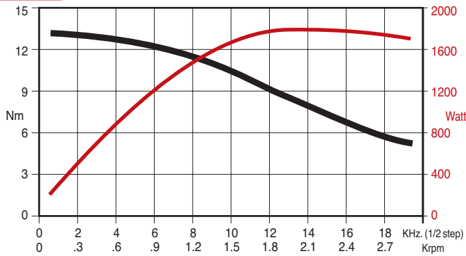
SANYO 103 H89222 6541 - bipolar connection RTA BCW02 drive
