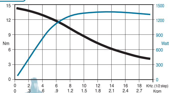
SANYO 103 8960 6551 - parallel bipolar connection RTA BCW02 drive
