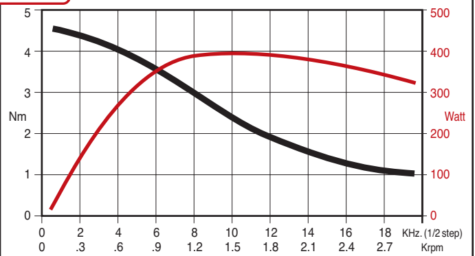
SANYO 103 H8222 6340 - bipolar connection RTA GMD04 drive
