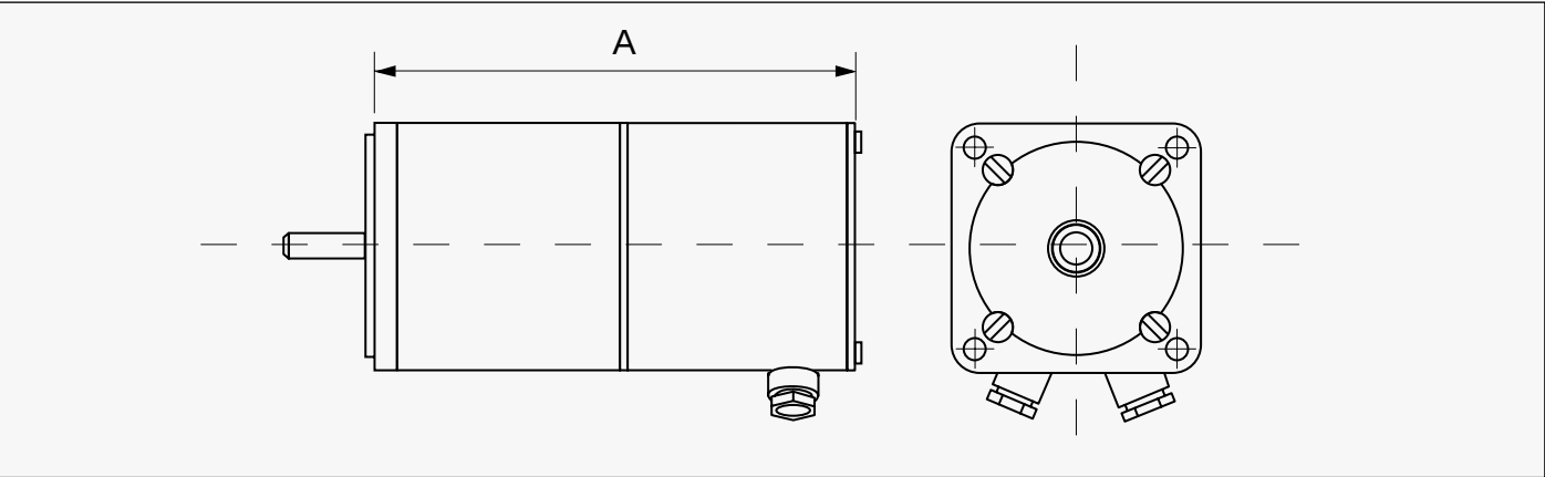
Dimensions stepping motor with gear box, encoder and brake
