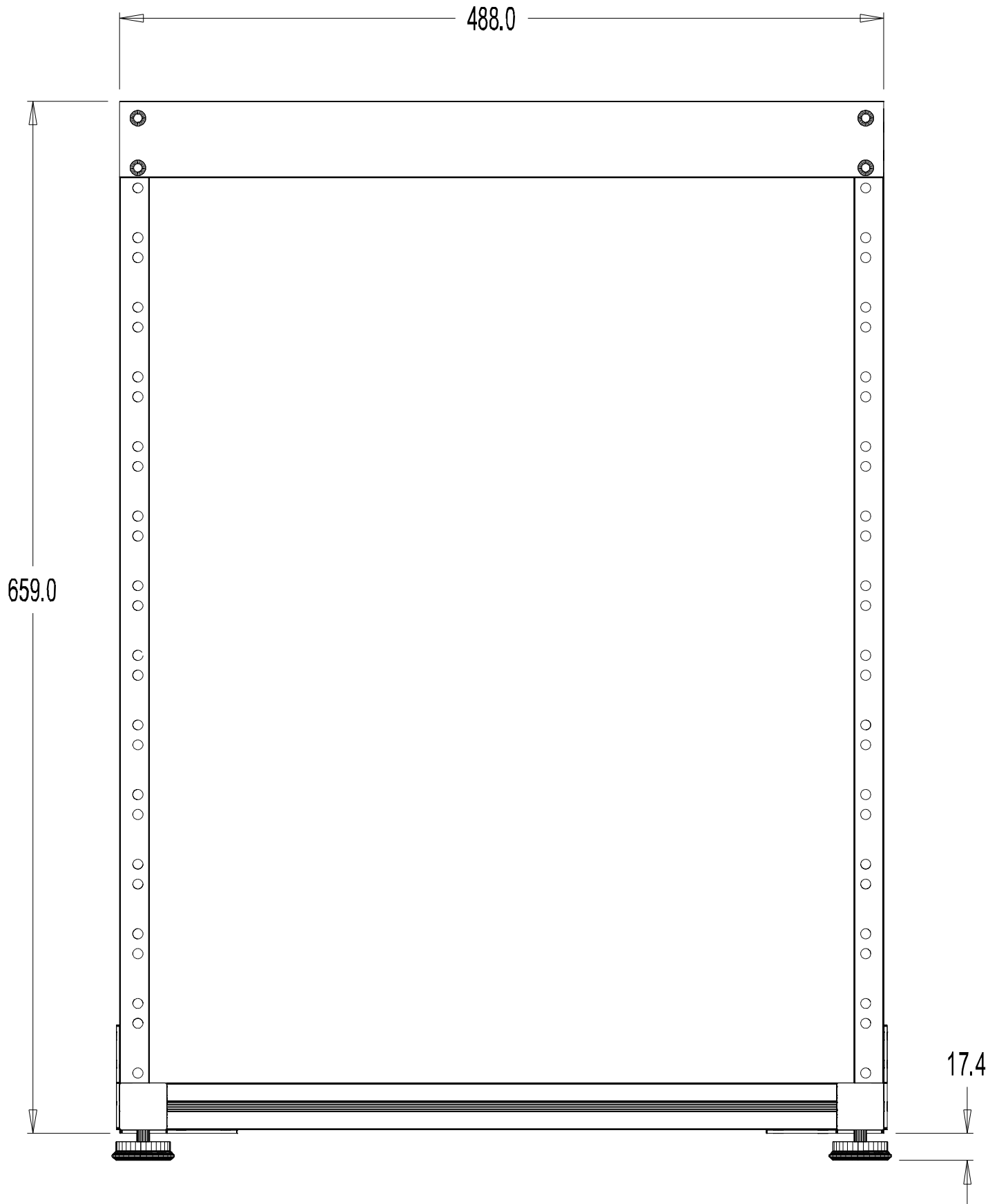
RF-14U-TS30 Front View (View 6 Level 106)
