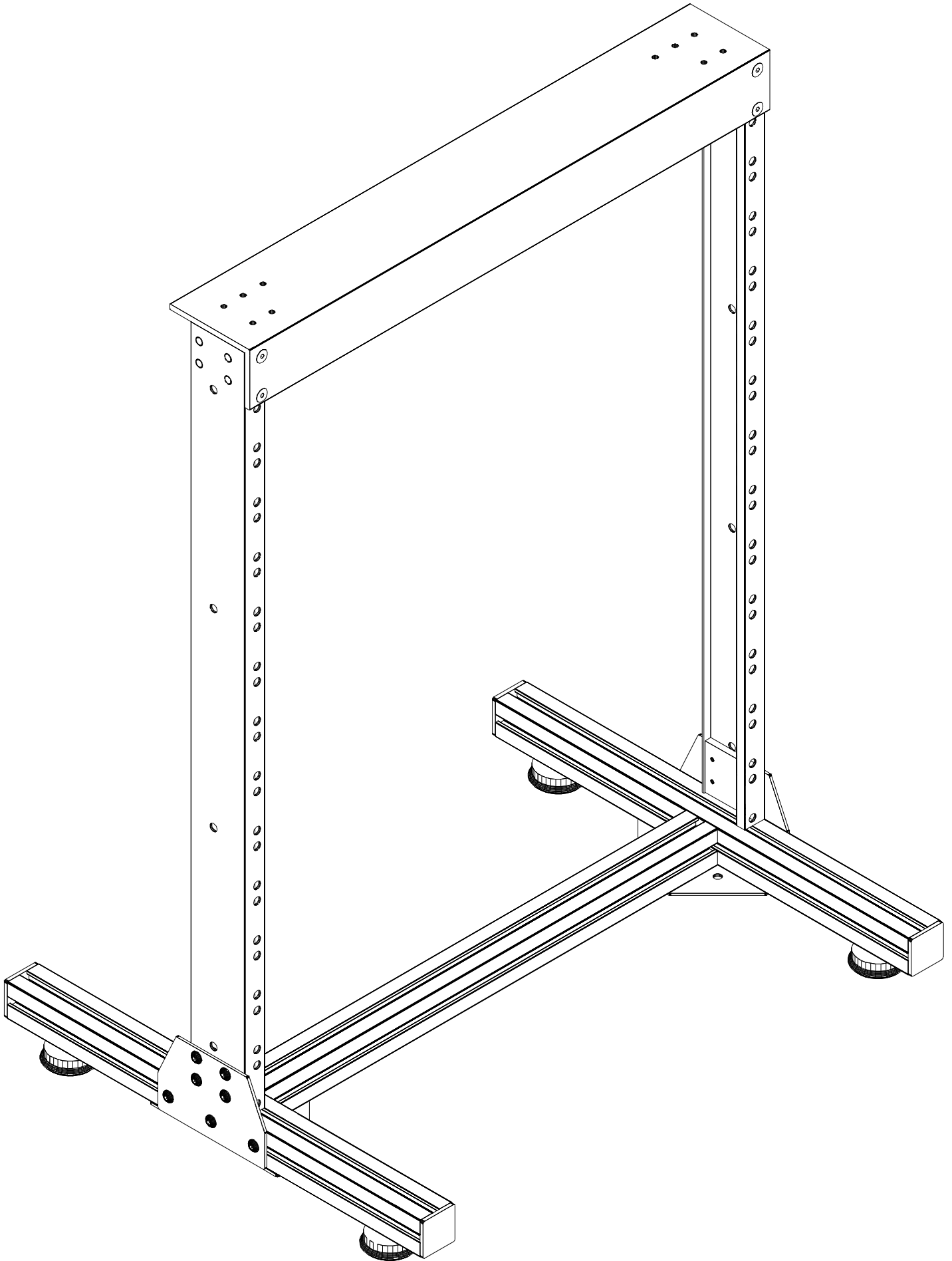
RF-14U-TS30-Assy.Prt (V7L166-Fasteners)
