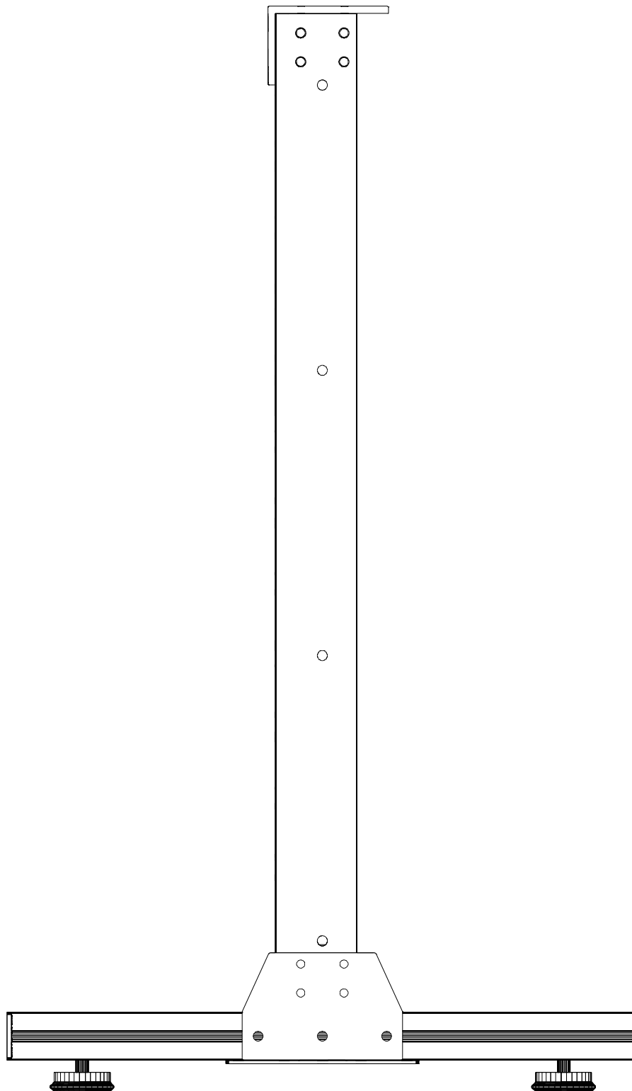
RF-14U-TS30 Side View (View 2 Level 102)
