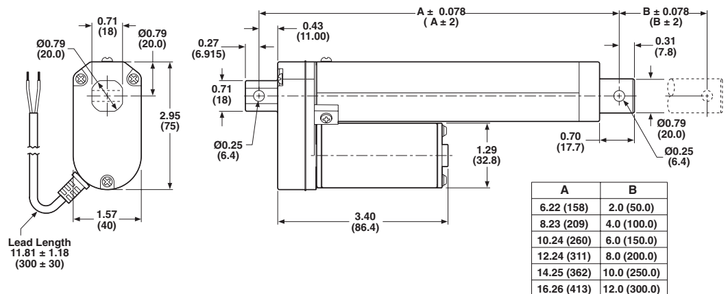
With Limit Switch Only
