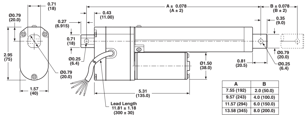
With Limit Switches and Potentiometer
