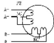
Figure 7: 6-lead motor full coil (higher torque) connections
