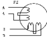
Figure 8: 8-lead motor series connections
