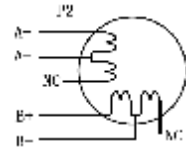
Figure 6: 6-lead motor half coil (higher speed) connections
