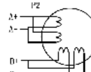
Figure 9: 8-lead motor parallel connections
