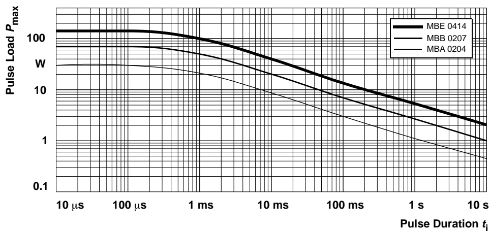
Maximum pulse load, single pulse; for permissible resistance change equivalent to 8000 h operation. Single Pulse
