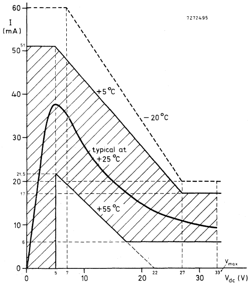
Fig. 7 Area of current/voltage characteristics.
