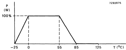
Fig. 4 Derating curve.
