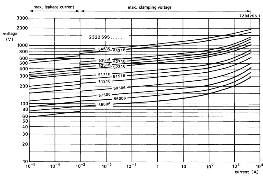
Fig. 12 V/I characteristics, 50/460 V, 595 series.
