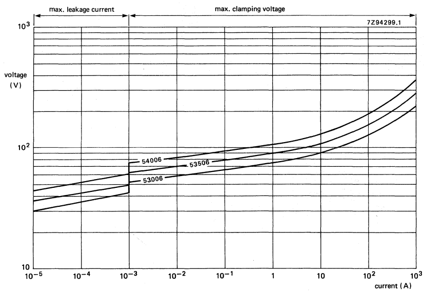
Fig. 11 V/I characteristics, 30/40 V, 595 series.
