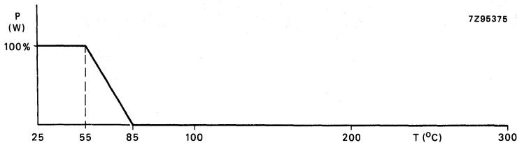
Fig. 2 Derating curve.
