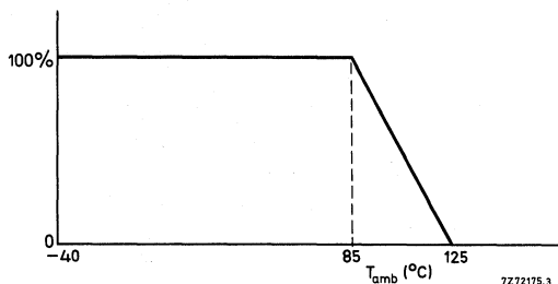
Fig. 2 Derating of max. d.c. and r.m.s. working voltage with temperature.
