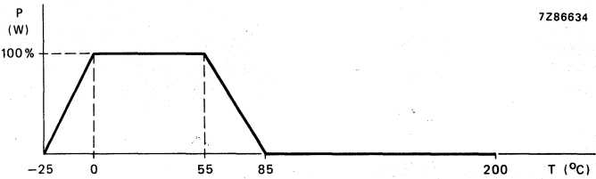
Fig. 2 Derating curve.
