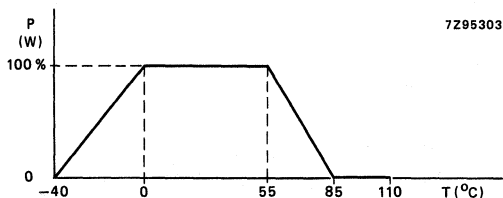
Fig. 3 Derating curve.
