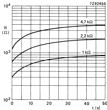
Fig. 6 Typical resistance/cooling time characteristics. Measured in still air at 25 °C. T_{\text{start}} = 85 \text{ °C} .
