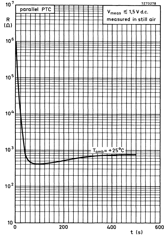
Fig. 10 Typical resistance versus cooling time characteristic of parallel PTC, T_{\text{start}} = 225^\circ\text{C} .
