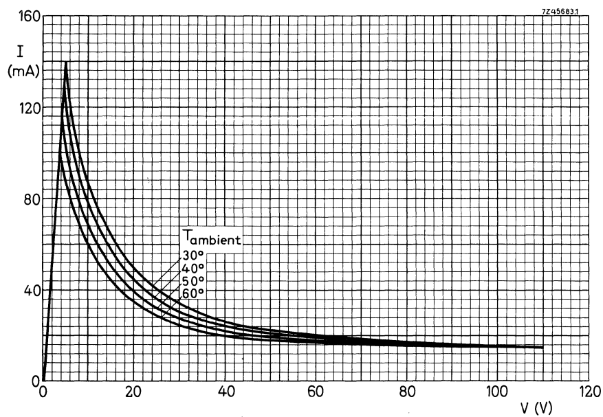
Fig. 2 Voltage/current characteristics of a PTC thermistor on a linear scale, with ambient temperature as a parameter.
