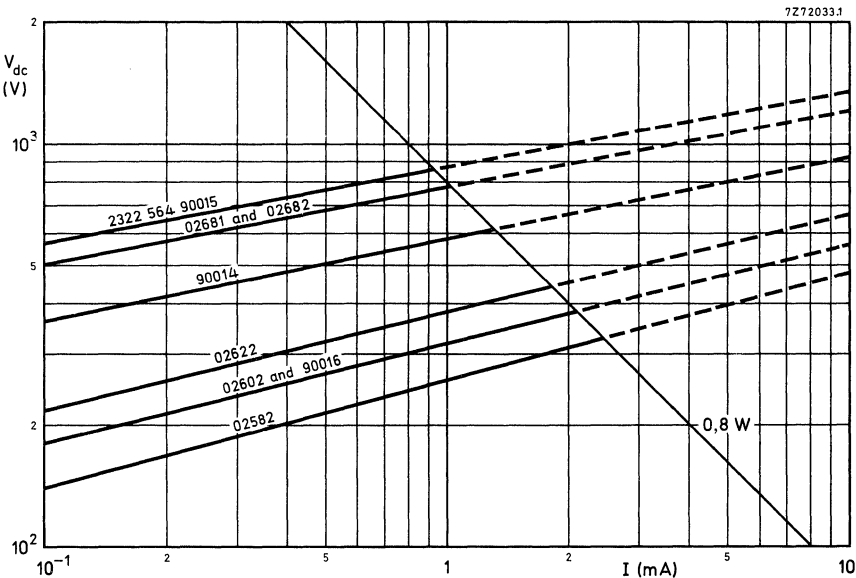
Fig. 2 Voltage/current characteristics.
