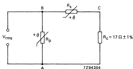
Fig. 2 Measuring circuit.
