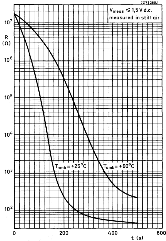
Fig. 9 Typical resistance versus cooling time characteristics of series PTC, T_{\text{start}} = 175^\circ\text{C} .
