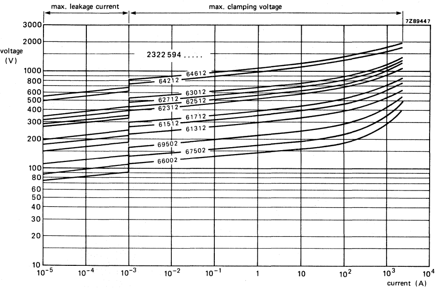
Fig. 2 V/I characteristics.
