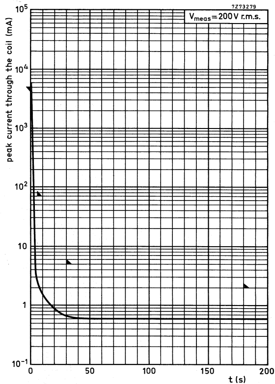
Fig. 12 Typical peak current through the coil versus time characteristic. Peak current limits are indicated by \blacktriangle . .
