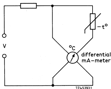
Fig. 13 Temperature measurement in cars. Cooling water measurements with bimetall or differential milliammeters.
