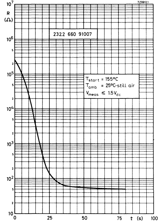
Fig. 6 Typical resistance/time (cooling) characteristic.
