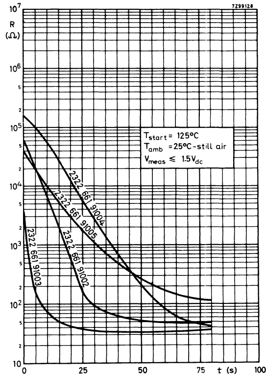
Fig. 3 Typical resistance/time (cooling) characteristics.
