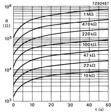
Fig. 6 Typical resistance/cooling time characteristics. Measured in still air at 25 °C. T_{\text{start}} = 85 \text{ °C} .
