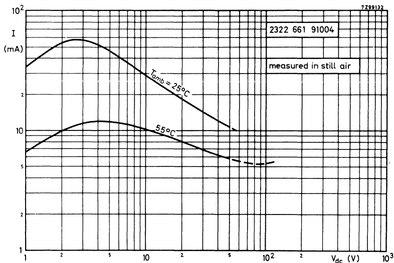
Fig. 6 Voltage/current characteristics.
