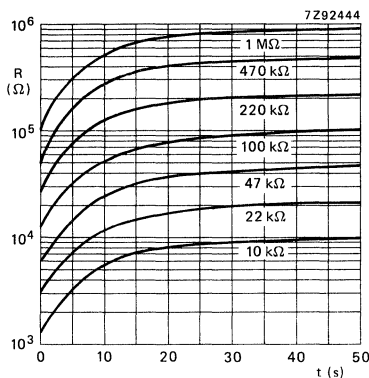
Fig. 6 Typical resistance/cooling time characteristics. Measured in still air at 25 °C. T_{start} = 85\text{ °C} .
