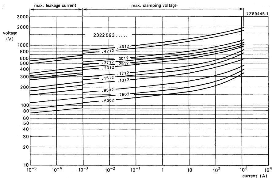
Fig. 2 V/I characteristics.
