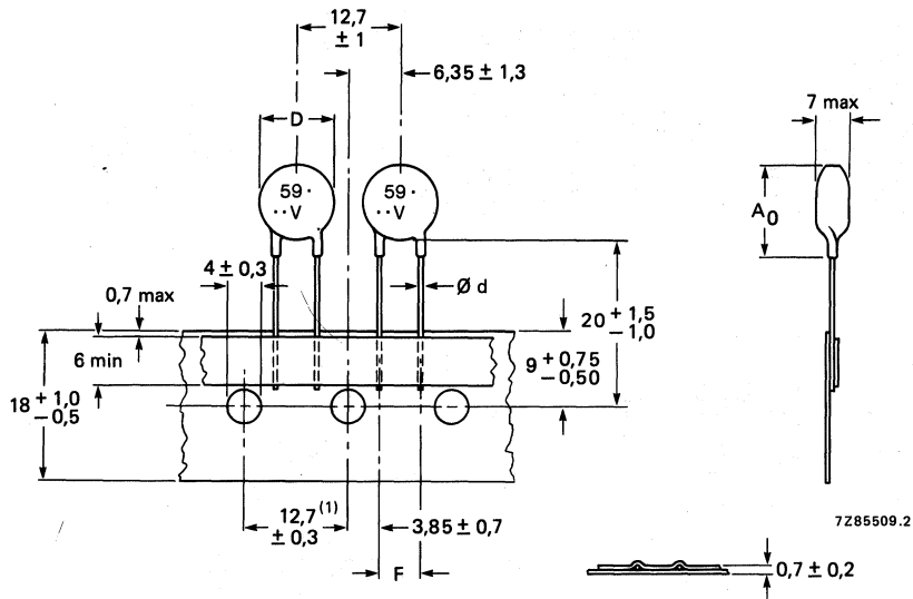
Fig. 3 Dimensions of bandolier, for dimensions of D , d , A_0 and F see Table 1.
