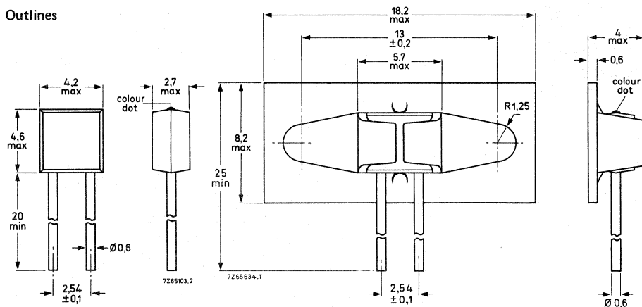
Fig.1 Type 2322 640 90013.
