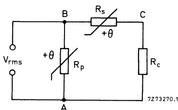
Fig. 2 Measuring circuit.
