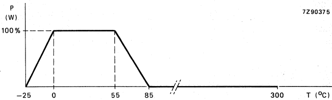
Fig. 2 Derating curve.
