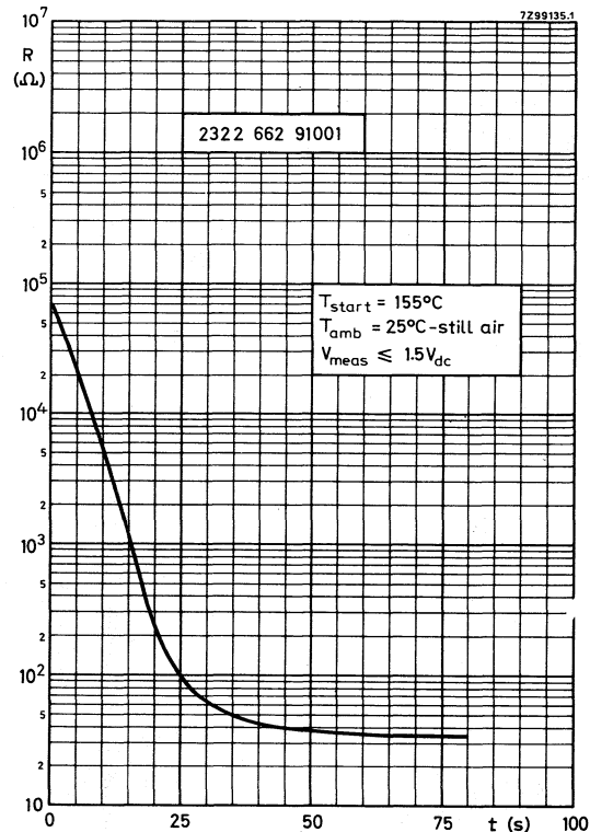
Fig. 4 Typical resistance/time (cooling) characteristic.
