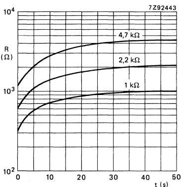
Fig. 6 Typical resistance/cooling time characteristics. Measured in still air at 25 °C. T_{start} = 85\text{ °C} .
