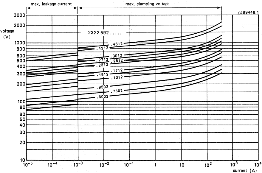
Fig. 2 V/I characteristics.
