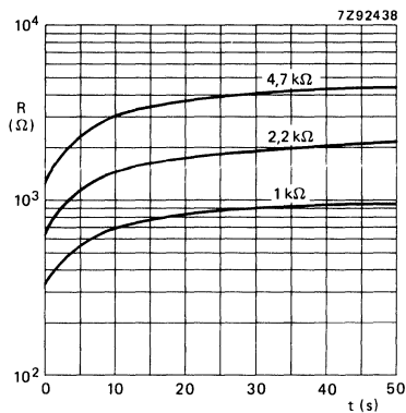
Fig. 5 Typical resistance/cooling characteristics. Measured in still air at 25 °C. T_{start} = 85^\circ\text{C} .
