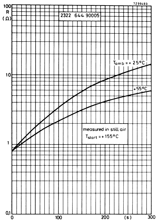
Fig. 7 Typical resistance/time (Cooling) characteristics.
