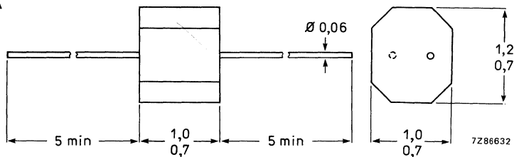
Fig. 1 version 2322 633 0....
