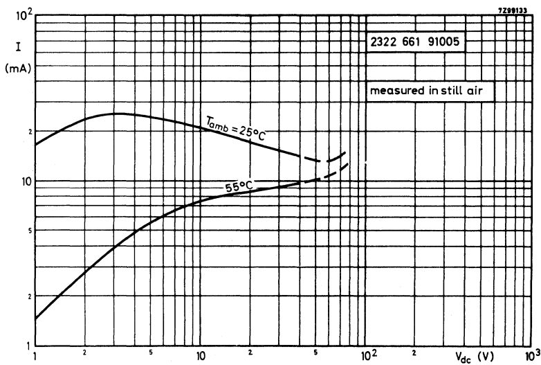
Fig. 7 Voltage/current characteristics.
