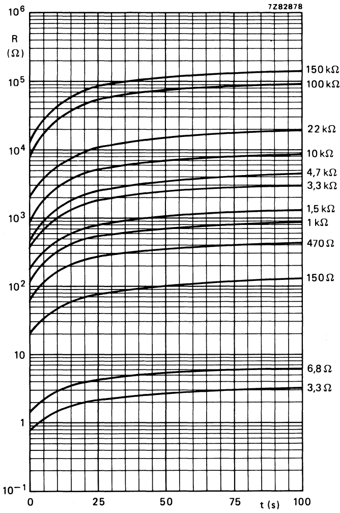
Fig. 8 Typical resistance/cooling time characteristic, T_{\text{amb}} = +25^\circ\text{C} , still air, T_{\text{start}} = +85^\circ\text{C} .
