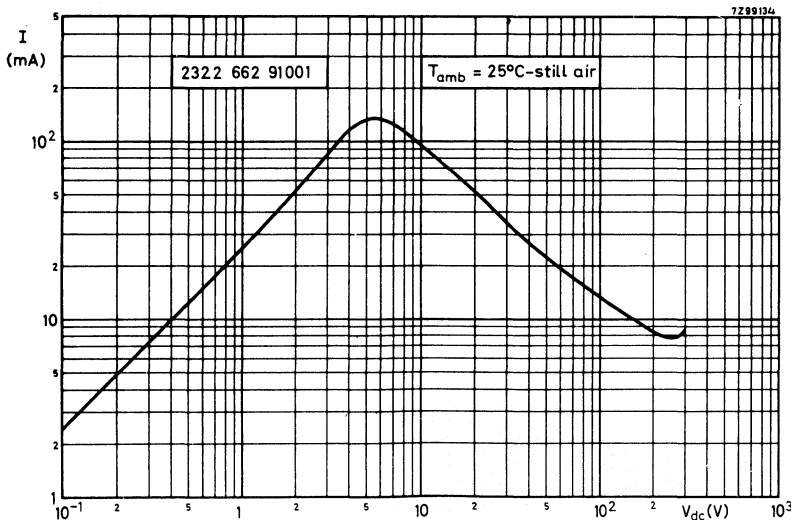
Fig. 2 Typical voltage/current characteristic.
