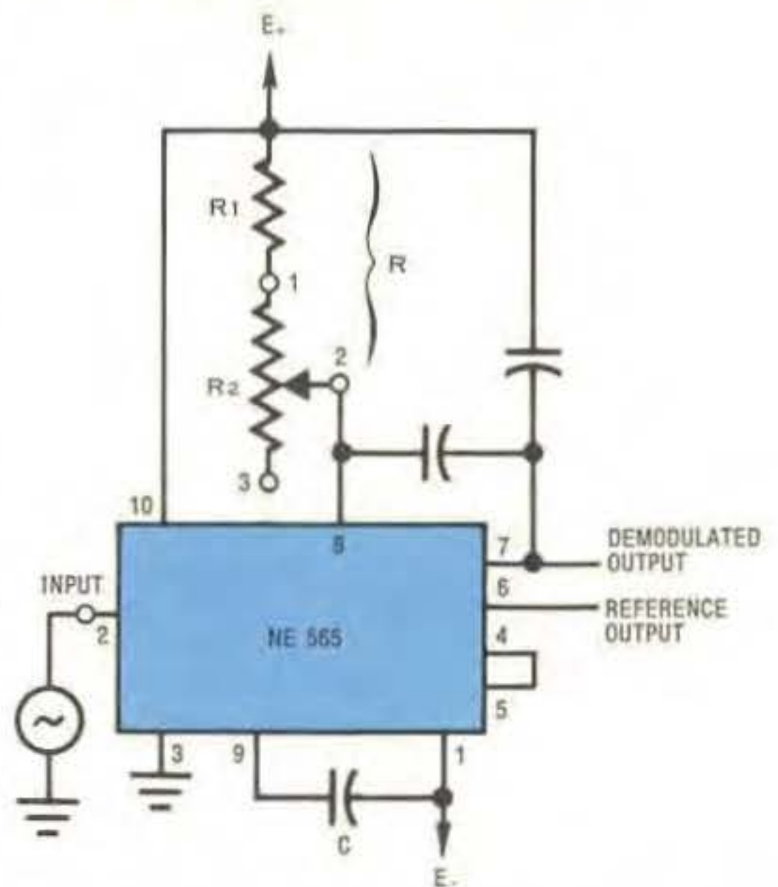
Fig. 4-18 Trimming potentiometers adjust free-run frequency in a phase locked loop FM demodulator
