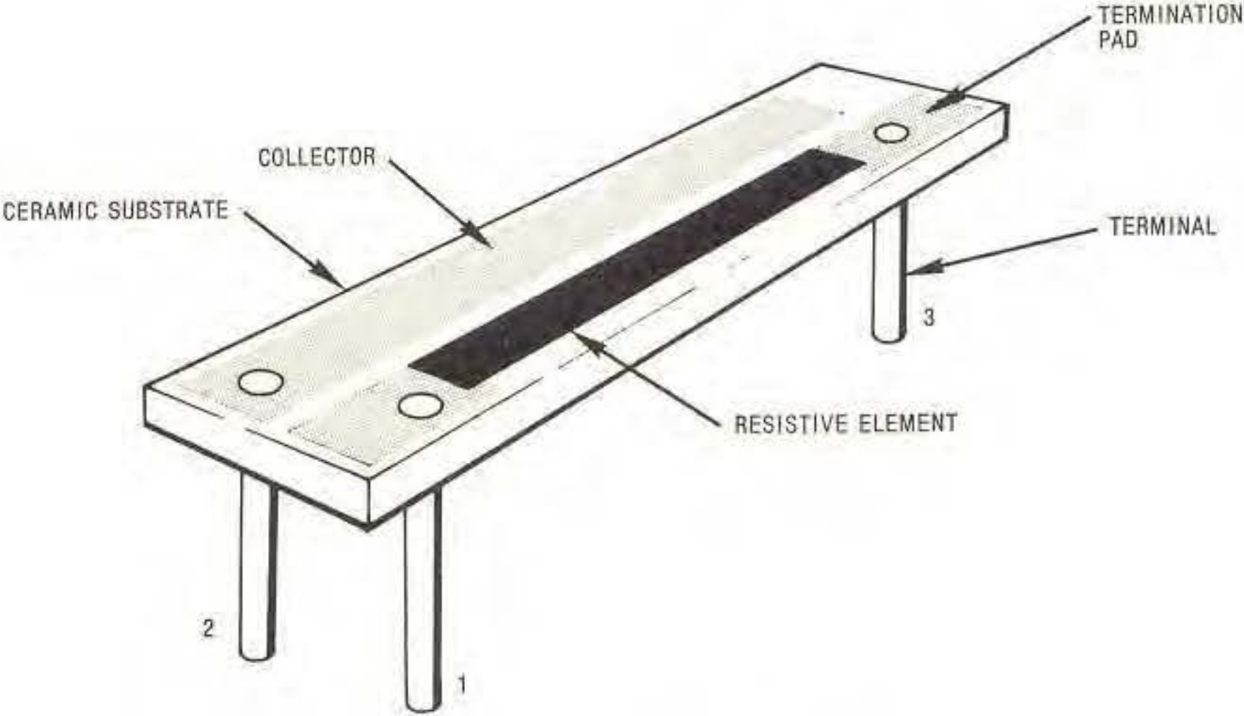
A. A COMMON CERMET POTENTIOMETER CONSTRUCTION
