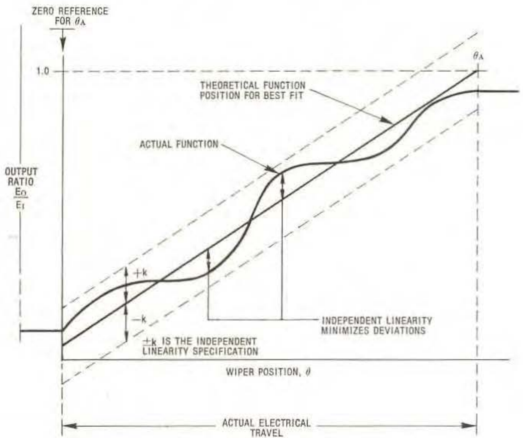
Fig. 2-35 Independent linearity
