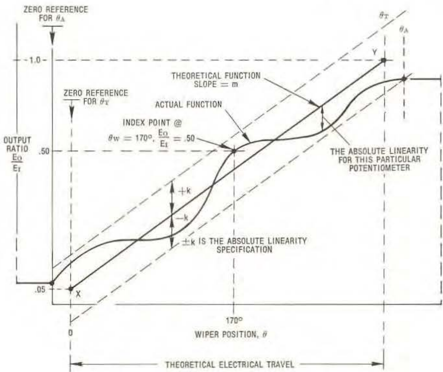
Fig. 2-34 Absolute linearity
