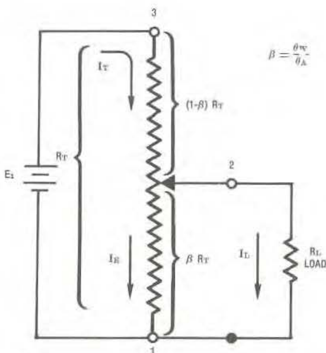
Fig. 6-11 A potentiometer with a loaded wiper circuit
