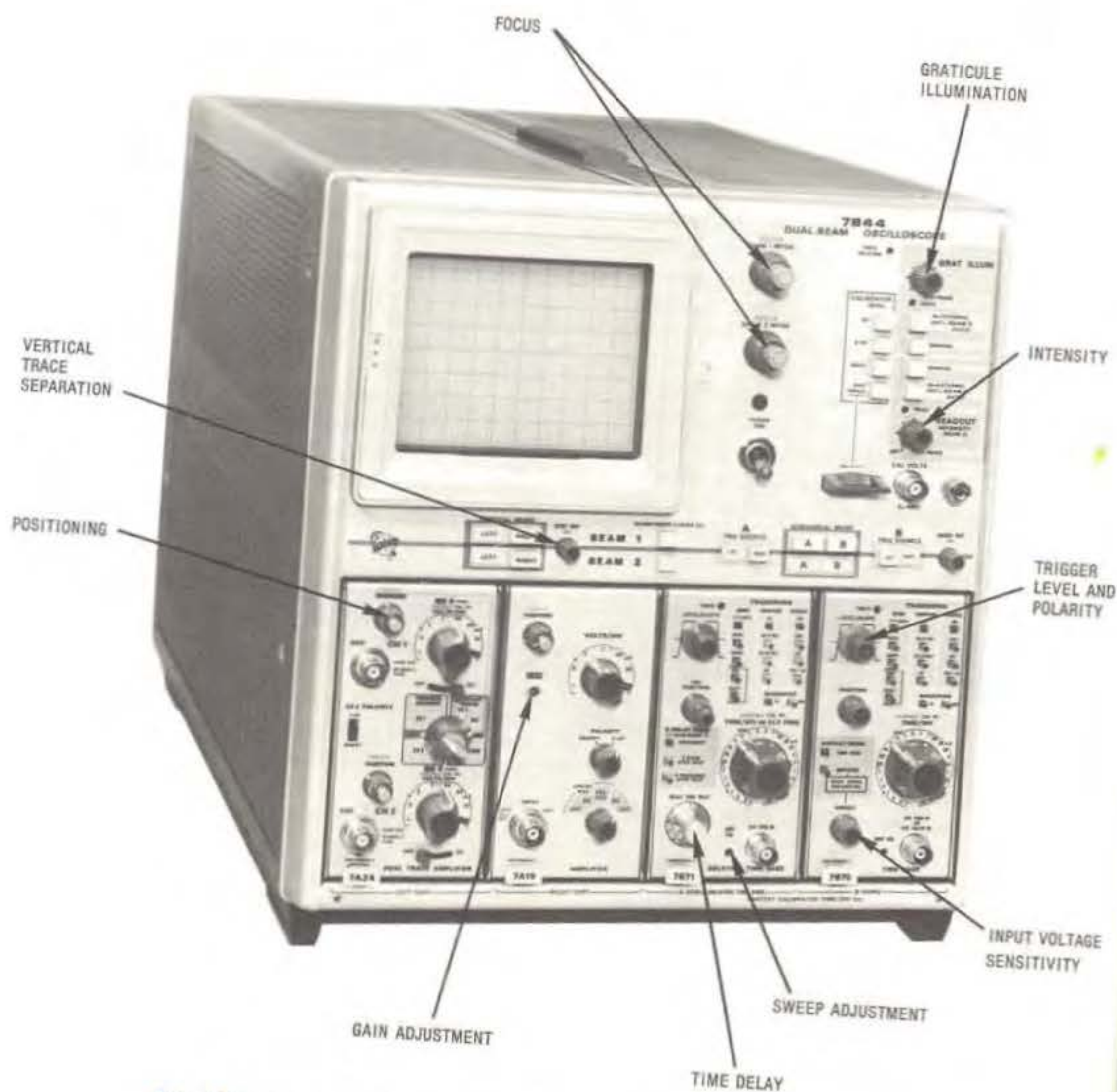
Fig. 5-4 Variable resistance controls contribute to the versatility of the modern test oscilloscope (Tektronix, Inc.)
