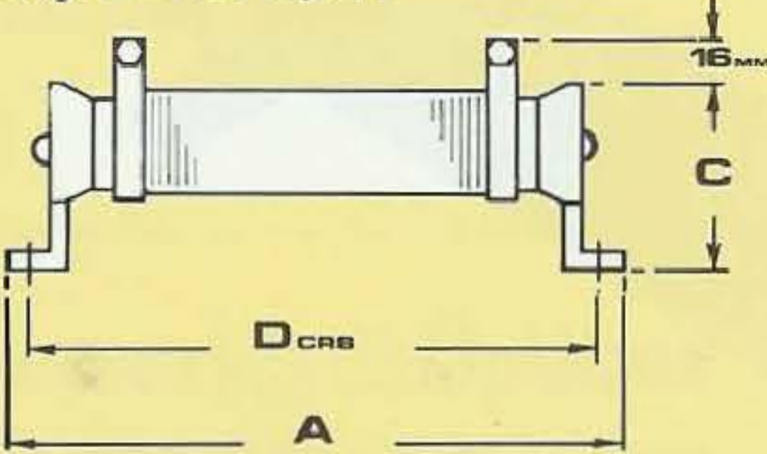
Single Tube Open
