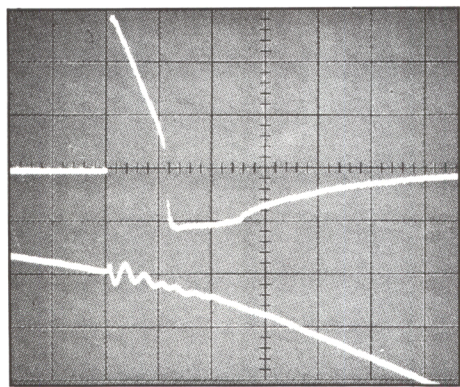
Oscilloscope illustrates a 3 kV fast rise time transient on top trace (1 kV/div and 80 us/div). Bottom trace with 5 V/div sensitivity illustrates the transient-killing ability of Philips line conditioners.
