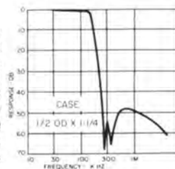
150 kHz Low Pass 3 db to 150 kHz, down 45 db above 250 kHz. 1500 ohms.
