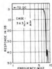
Low pass filter, 6 MHz. DC to 6 MHz within \pm 0.1 db. Attenuation at least 40 db at 8.5 MHz and higher. Source and load 75 ohms. Wt. approx. 8 oz.
