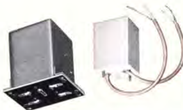
Special chopper type transformers with terminals or shielded leads; multiple high permeability magnetic shields; electrostatic shielding for voltage isolation of 2 \times 10^6 .
