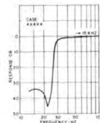
High pass filter, 30 Hz, used to eliminate from the output, 25 Hz sine wave pulses which control automatic programming on audio tracks of music tapes. Flat to 1 db from 50 Hz to 15 kHz, within 3 db to 30 Hz. Attenuation of at least 35 db from 25 Hz to 20 Hz. Source and load 600 ohms. Wt. approx. 6 lbs. MIL-F-18327C.
