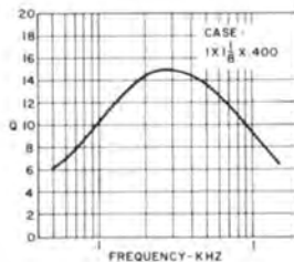
Flat low frequency 50 henries inductor only .400 high. Q of 10 at 100 Hz. DCR 2360 ohms. Grade 4, MIL-T-27C.
