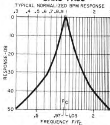
TYPICAL NORMALIZED BPM RESPONSE
