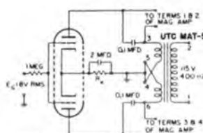
FIG. 3 PARALLEL GRIDS-PUSH-PULL PLATES
