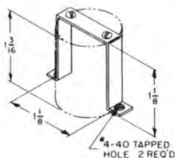
O-BR Ouncer chassis mount bracket
