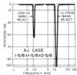
Band reject filters (two shown). The 1050 Hz filter has 50 db attenuation at center frequency and is only 3 db down at 950 and 1150 Hz. The 12.75 kHz filter has more than 100 db attenuation at center frequency and is only 3 db down at 10.8 kHz and 15 kHz. Source and load for each filter 600 ohms, both are MIL-F-18327C. Wt. 0.7 lbs.
