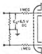
FIG. 2 GRID CIRCUIT MODIFICATION FOR DC INPUT
