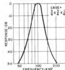
Ultra-miniature 100 kHz band pass filter only 1/4" high. Within 3 db 90 kHz to 110 kHz. Attenuation of at least 45 db at 50 kHz and at 200 kHz. Source and load 10K ohms.
