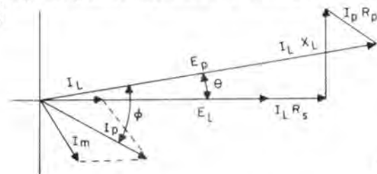
Vector Diagram
