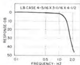
One Hz low pass filter. Flat to 1 db up to 0.75 Hz, within 2 db up to 1 Hz. Attenuation of at least 40 db for frequencies above 2 Hz. Source and load 10K ohms. MIL-F-18327C. Wt. 6 lbs.
