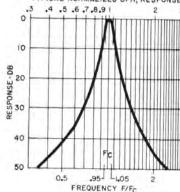
TYPICAL NORMALIZED BPM RESPONSE
