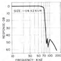
Ultra-miniature low pass filter only 1/4" high. DC to 40 kHz within \pm 0.1 db, within 1 db to 60 kHz, 3 db to 70 kHz. Attenuation of at least 40 db above 81 kHz. Source and load 1K ohms, MIL-F-18327C. Wt. 1.2 ounces.
