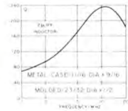
Type FD, 2 microhenry temperature stable miniature inductor. High Q in the 2 MHz to 20 MHz frequency range. Supplied in either epoxy case (23/32 dia x 1/2" high) Grade 5 or metal case (11/16 dia x 9/16" long) Grade 4. MIL-T-27C.
