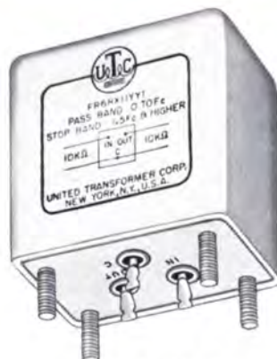
FILTER CASE M
