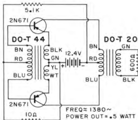
TYPICAL CIRCUIT OF STOCK DO-T UNITS FOR SPECIAL CONVERTER APPLICATION
