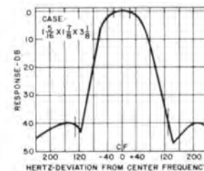
Miniaturized receiving filters, available from 425 Hz to 3315 Hz. Within 3 db at \pm 42.5 Hz and attenuation of at least 36 db at \pm 130 Hz. Source and load 600 ohms. Wt. approx. 3/4 lbs.
