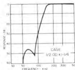
150 kHz High Pass 3 db to 150 kHz, down 45 db below 85 kHz. 7500 ohms
