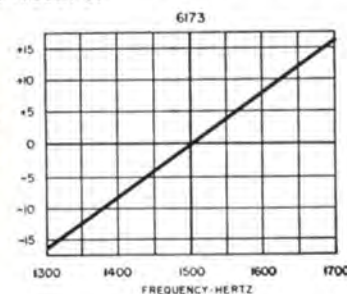
UTC high Q discriminators provide exceptional amplification and linearity. Values are volts. 1\frac{1}{16} " x 1\frac{1}{8} " x 3".
